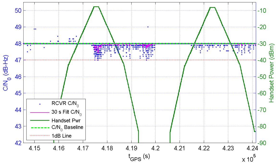
Receiver 113 Average C/N 0 for All Channels and Handset Power at Receiver for TE16/17
