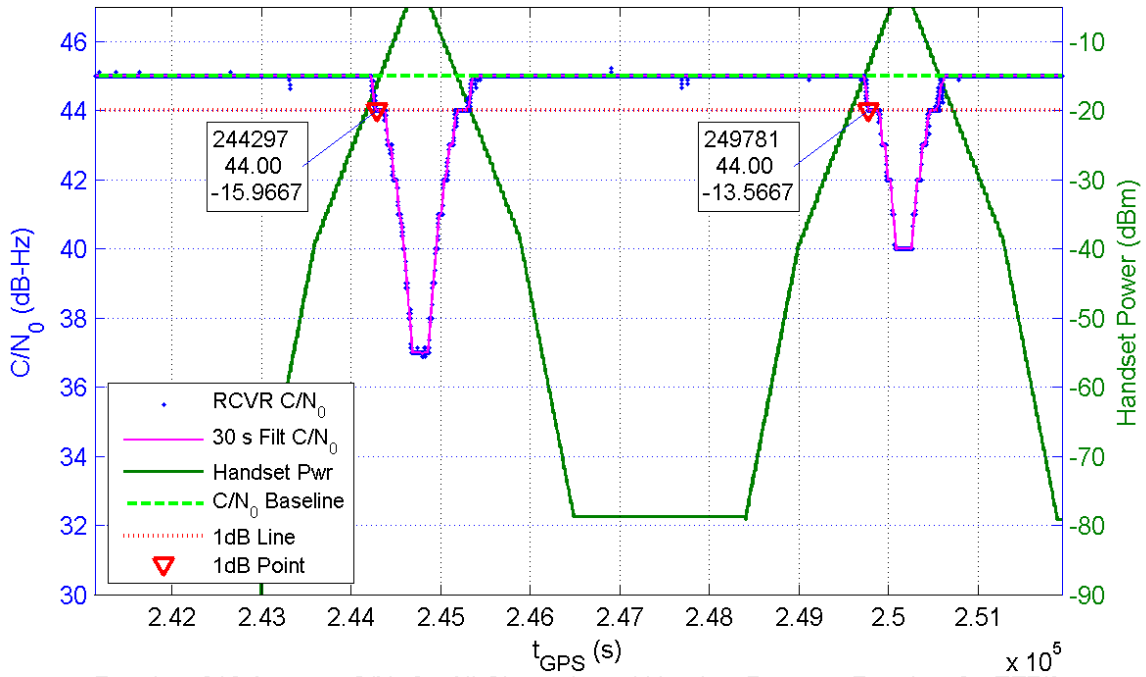
Receiver 316 Average C/N_0 for All Channels and Handset Power at Receiver for TE7/8
