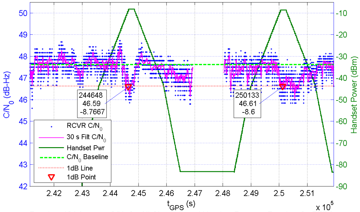
Receiver 124 Average C/N_0 for All Channels and Handset Power at Receiver for TE7/8
