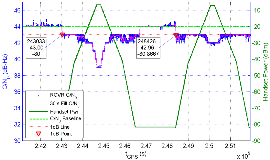
Receiver 249 Average C/N_0 for All Channels and Handset Power at Receiver for TE7/8
