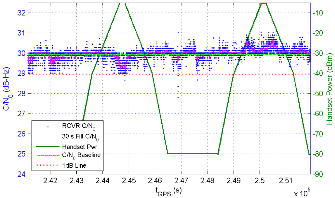
Receiver 377 Average C/N_0 for All Channels and Handset Power at Receiver for TE7/8
