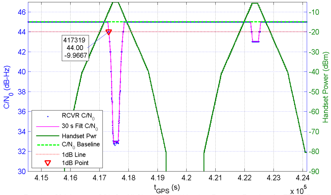
Receiver 234 Average C/N_0 for All Channels and Handset Power at Receiver for TE16/17
