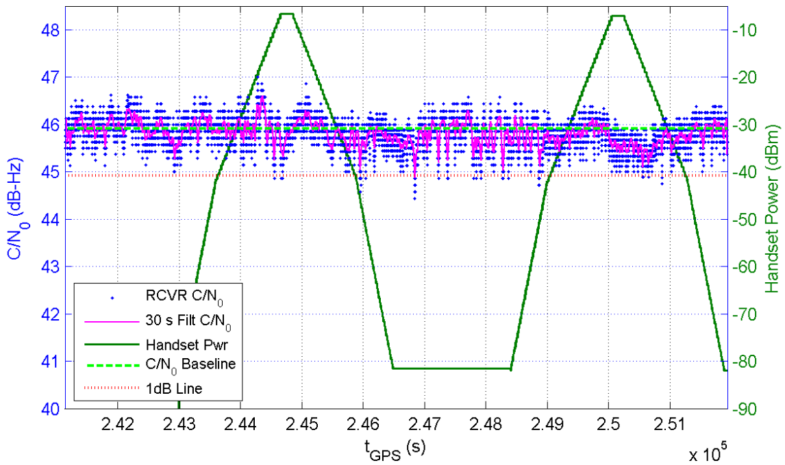
Receiver 396 Average C/N_0 for All Channels and Handset Power at Receiver for TE7/8
