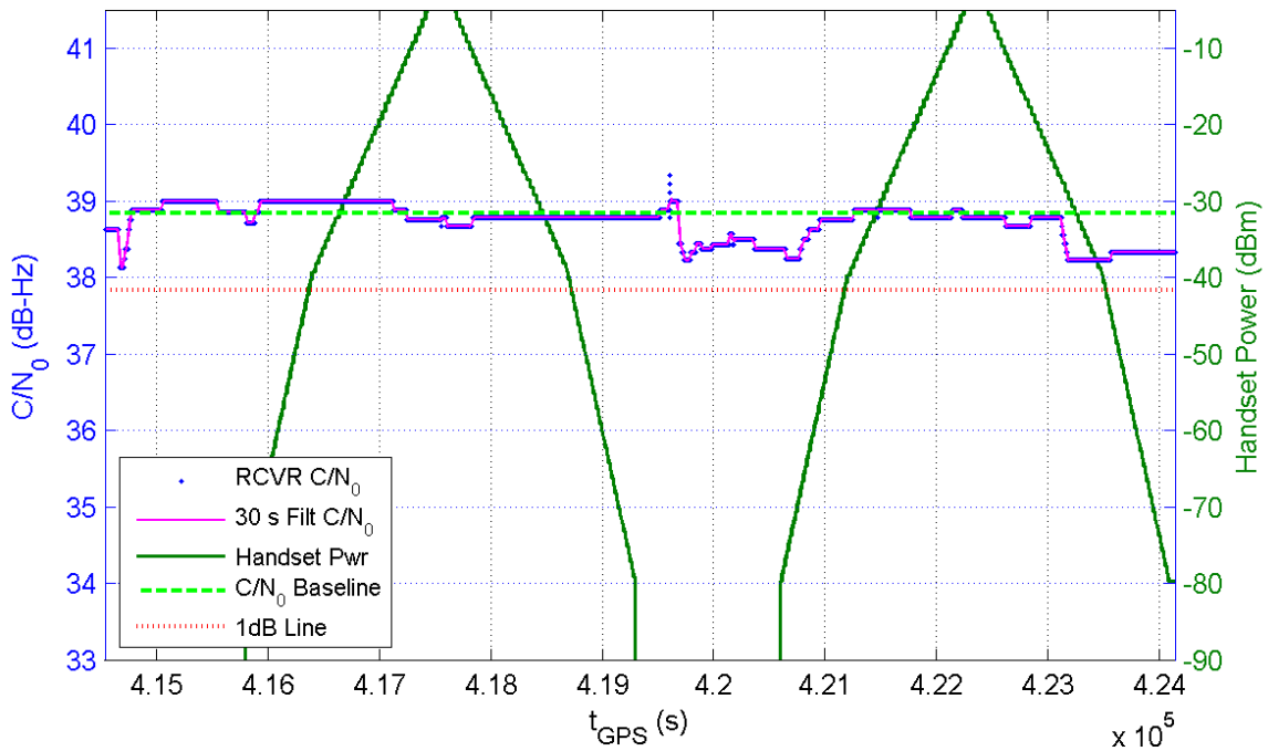
Receiver 352 Average C/N_0 for All Channels and Handset Power at Receiver for TE16/17
