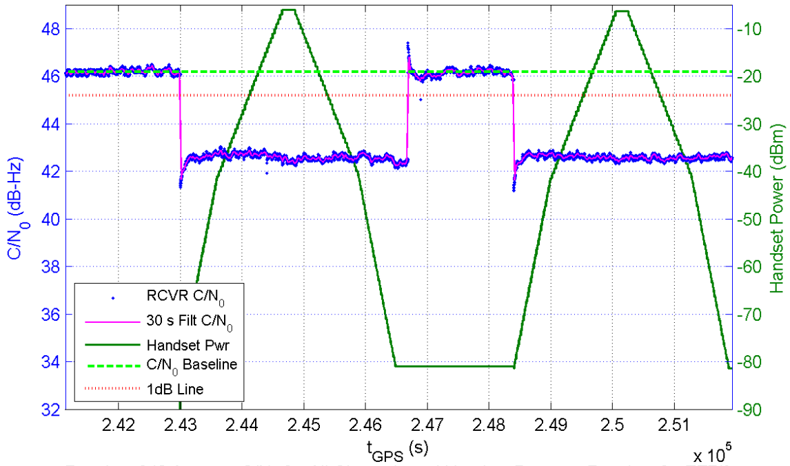
Receiver 340 Average C/N_0 for All Channels and Handset Power at Receiver for TE7/8
