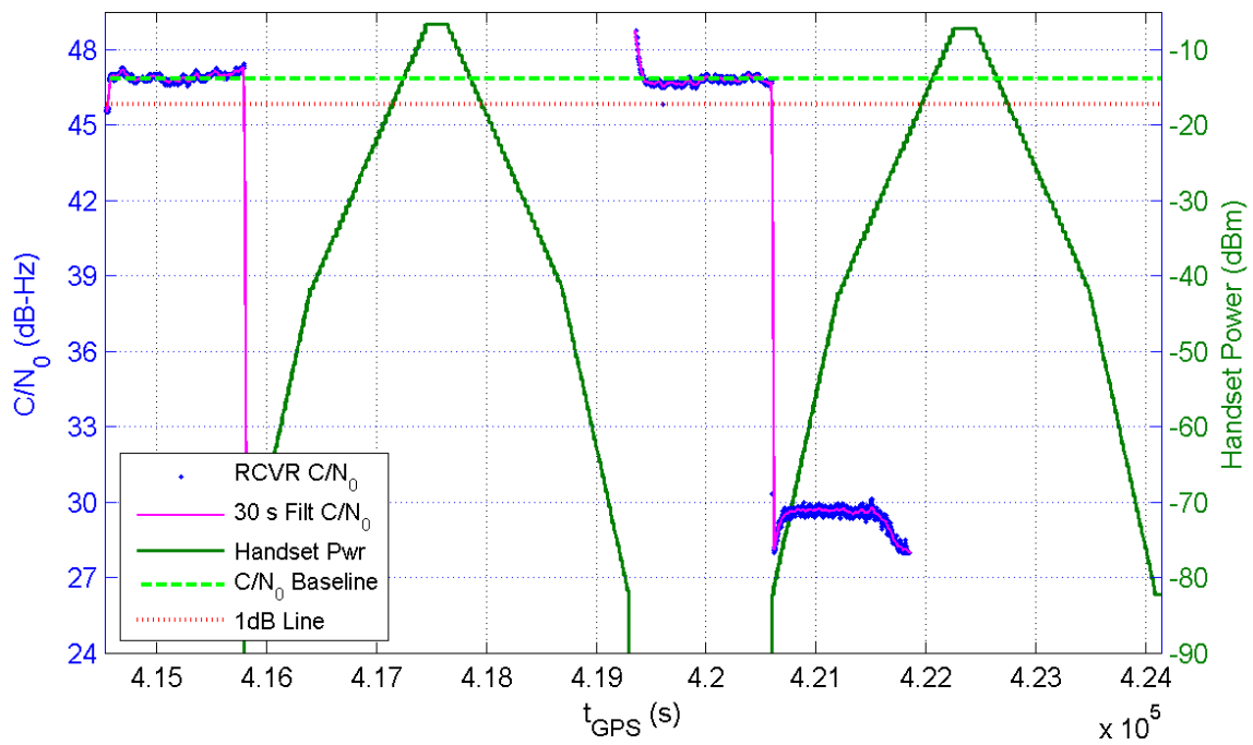
Receiver 215 Average C/N_0 for All Channels and Handset Power at Receiver for TE16/17
