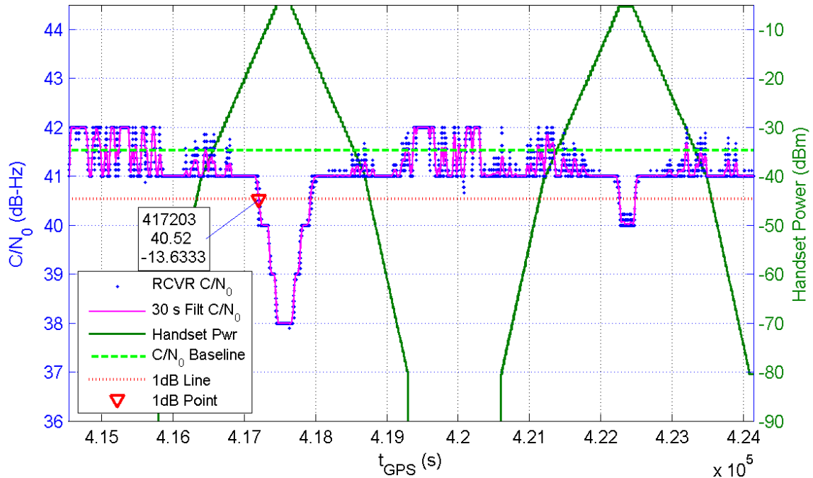
Receiver 104 Average C/N_0 for All Channels and Handset Power at Receiver for TE16/17
