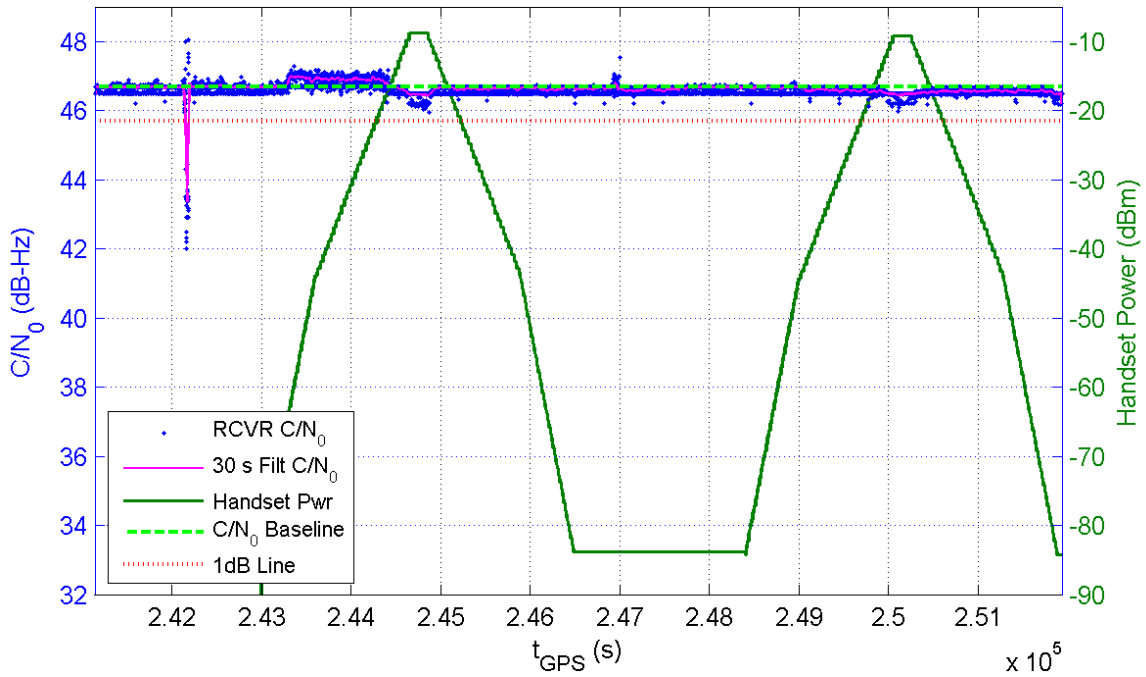
Receiver 118 Average C/N_0 for All Channels and Handset Power at Receiver for TE7/8
