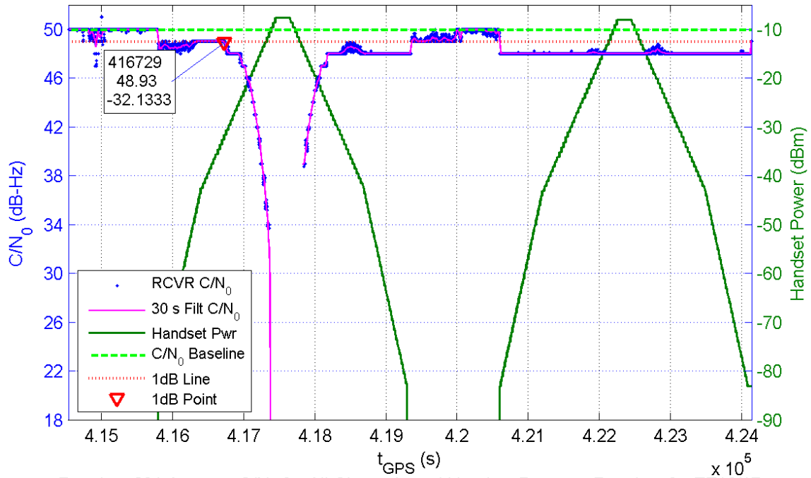
Receiver 231 Average C/N 0 for All Channels and Handset Power at Receiver for TE16/17
