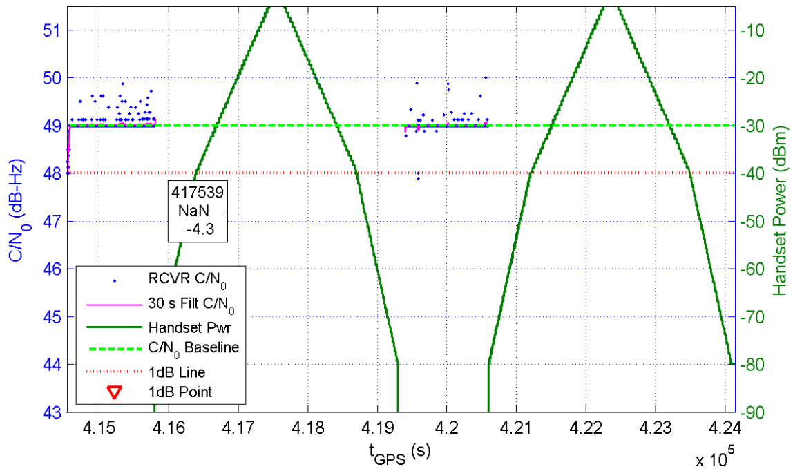
Receiver 121 Average C/N_0 for All Channels and Handset Power at Receiver for TE16/17
