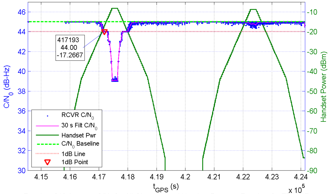
Receiver 318 Average C/N_0 for All Channels and Handset Power at Receiver for TE16/17
