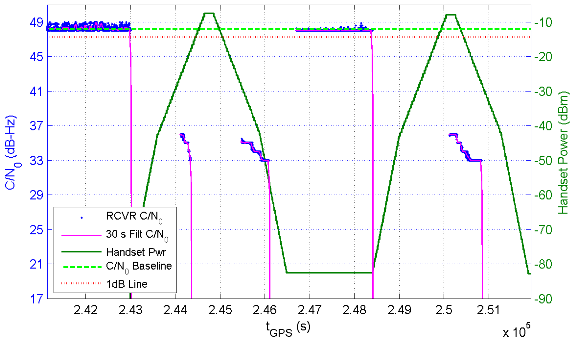
Receiver 382 Average C/N_0 for All Channels and Handset Power at Receiver for TE7/8
