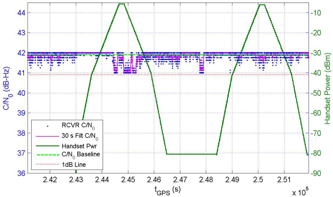
Receiver 132 Average C/N_0 for All Channels and Handset Power at Receiver for TE7/8
