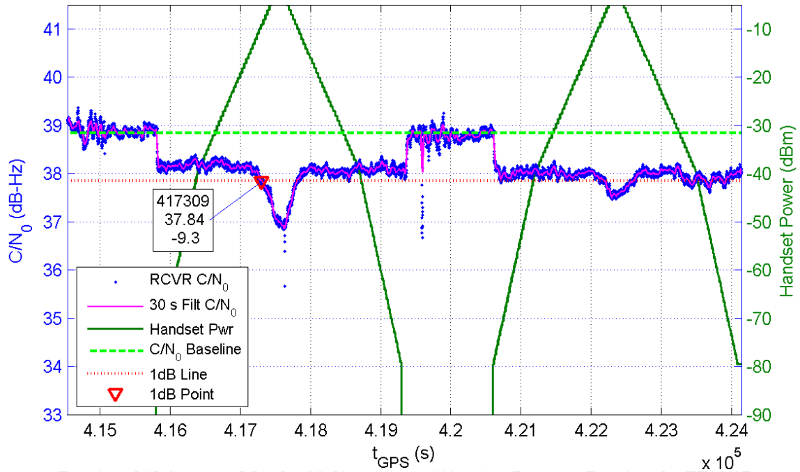
Receiver 212 Average C/N_0 for All Channels and Handset Power at Receiver for TE16/17
