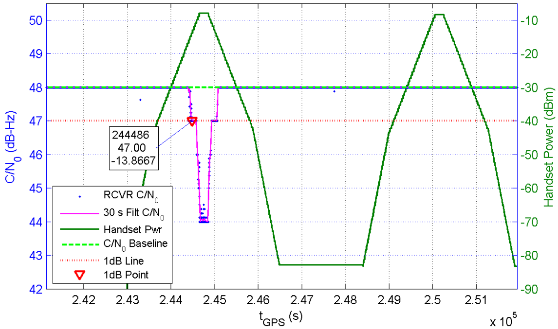
Receiver 116 Average C/N_0 for All Channels and Handset Power at Receiver for TE7/8
