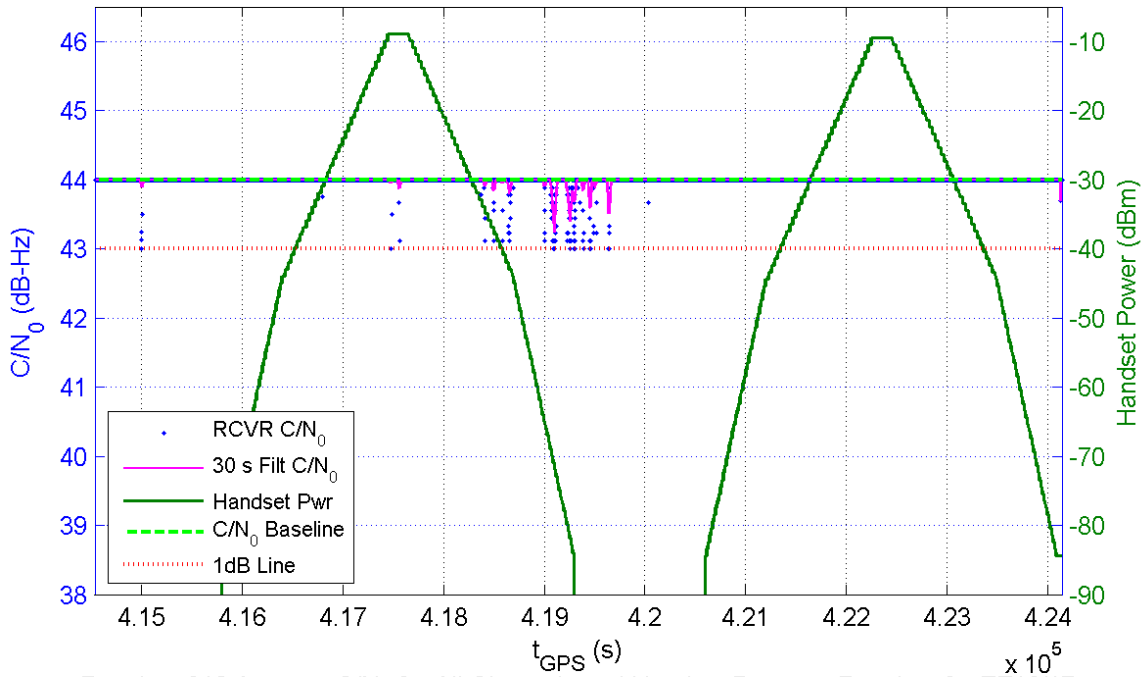
Receiver 310 Average C/N_0 for All Channels and Handset Power at Receiver for TE16/17
