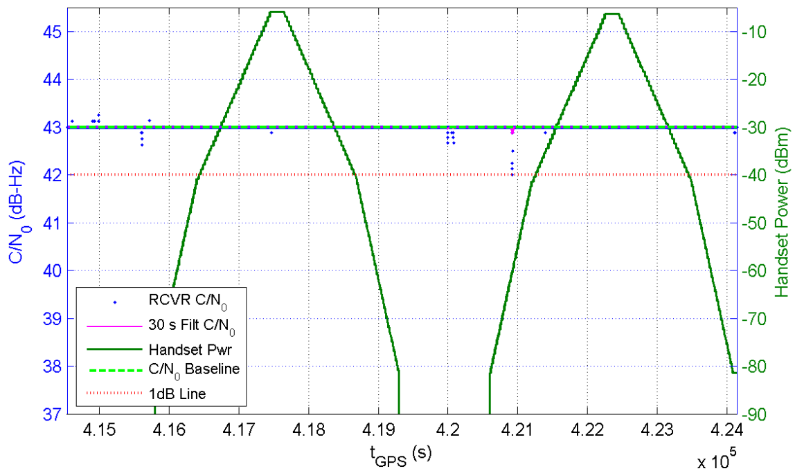
Receiver 397 Average C/N_0 for All Channels and Handset Power at Receiver for TE16/17
