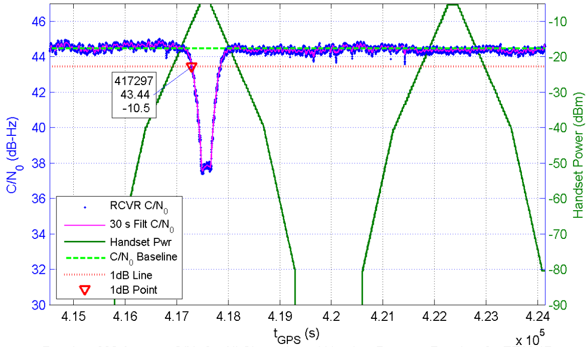
Receiver 392 Average C/N_0 for All Channels and Handset Power at Receiver for TE16/17
