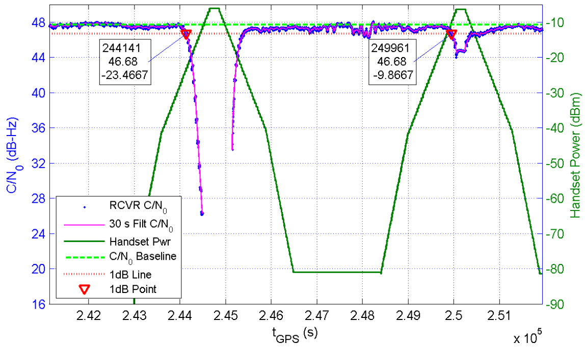
Receiver 399 Average C/N_0 for All Channels and Handset Power at Receiver for TE7/8
