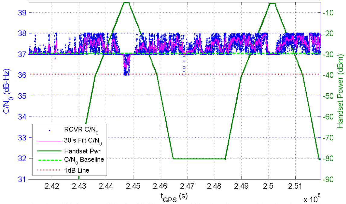
Receiver 388 Average C/N_0 for All Channels and Handset Power at Receiver for TE7/8
