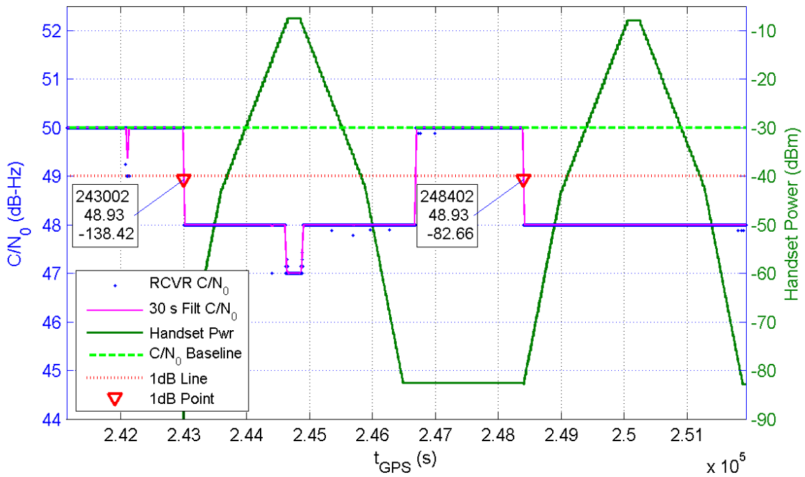
Receiver 331 Average C/N_0 for All Channels and Handset Power at Receiver for TE7/8
