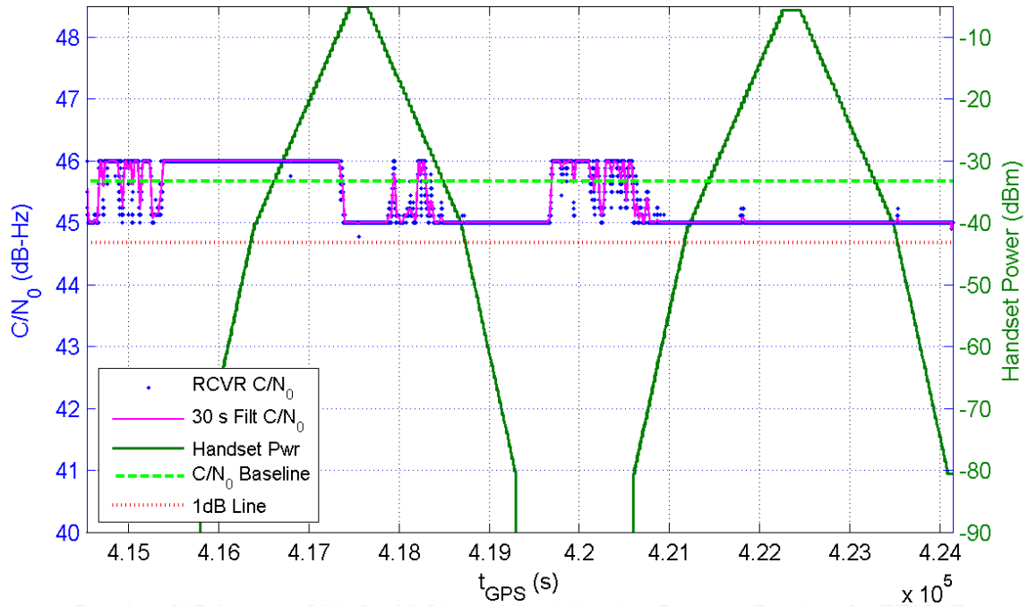
Receiver 347 Average C/N_0 for All Channels and Handset Power at Receiver for TE16/17
