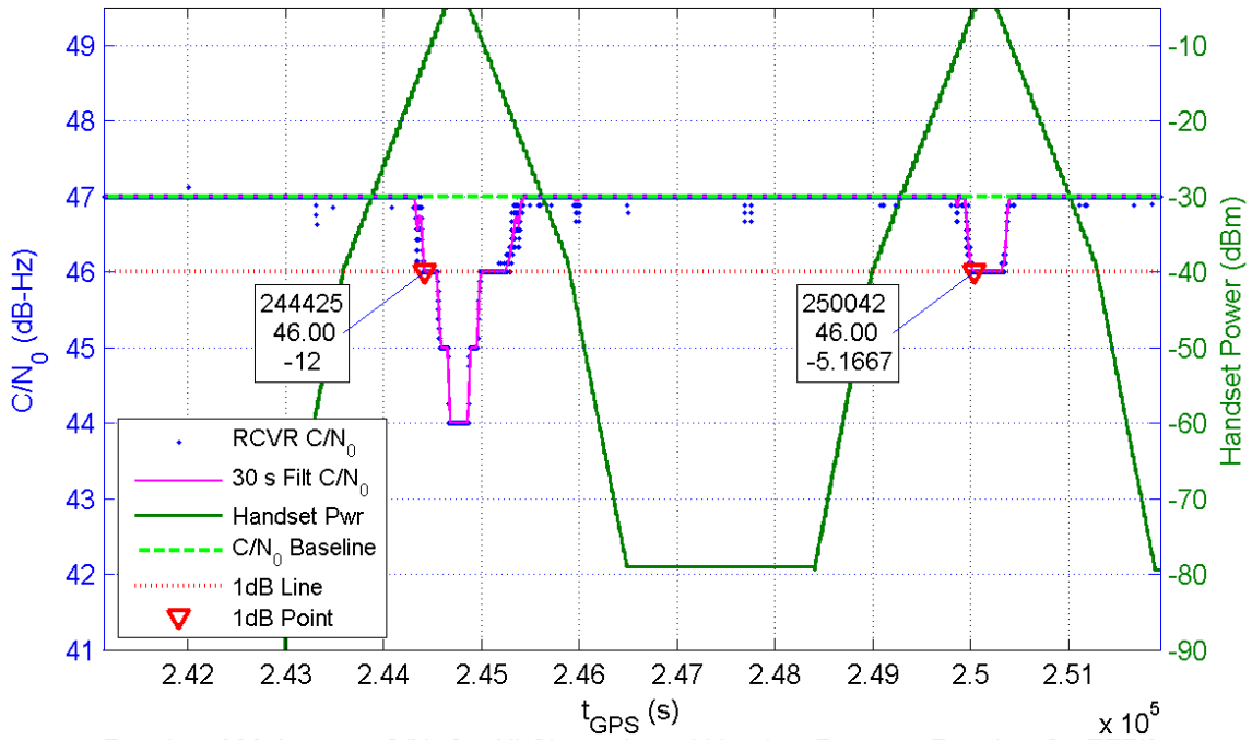
Receiver 338 Average C/N_0 for All Channels and Handset Power at Receiver for TE7/8
