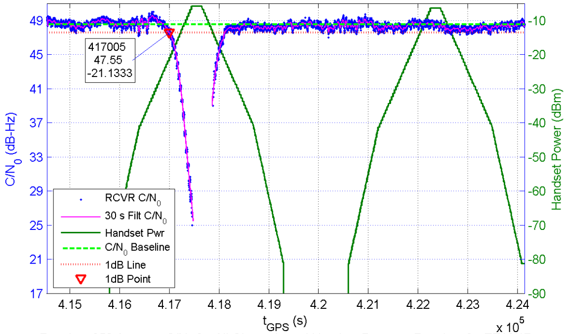
Receiver 352 Average C/N_0 for All Channels and Handset Power at Receiver for TE16/17
