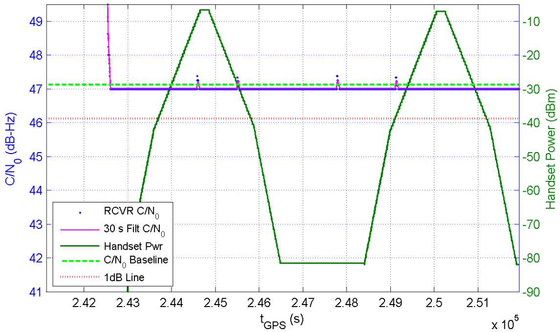
Receiver 340 Average C/N_0 for All Channels and Handset Power at Receiver for TE7/8
