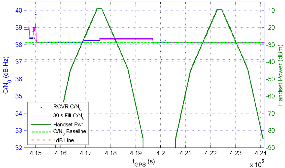
Receiver 129 Average C/N_0 for All Channels and Handset Power at Receiver for TE16/17
