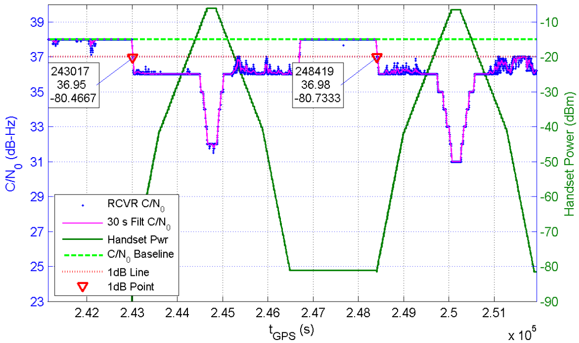
Receiver 320 Average C/N_0 for All Channels and Handset Power at Receiver for TE7/8
