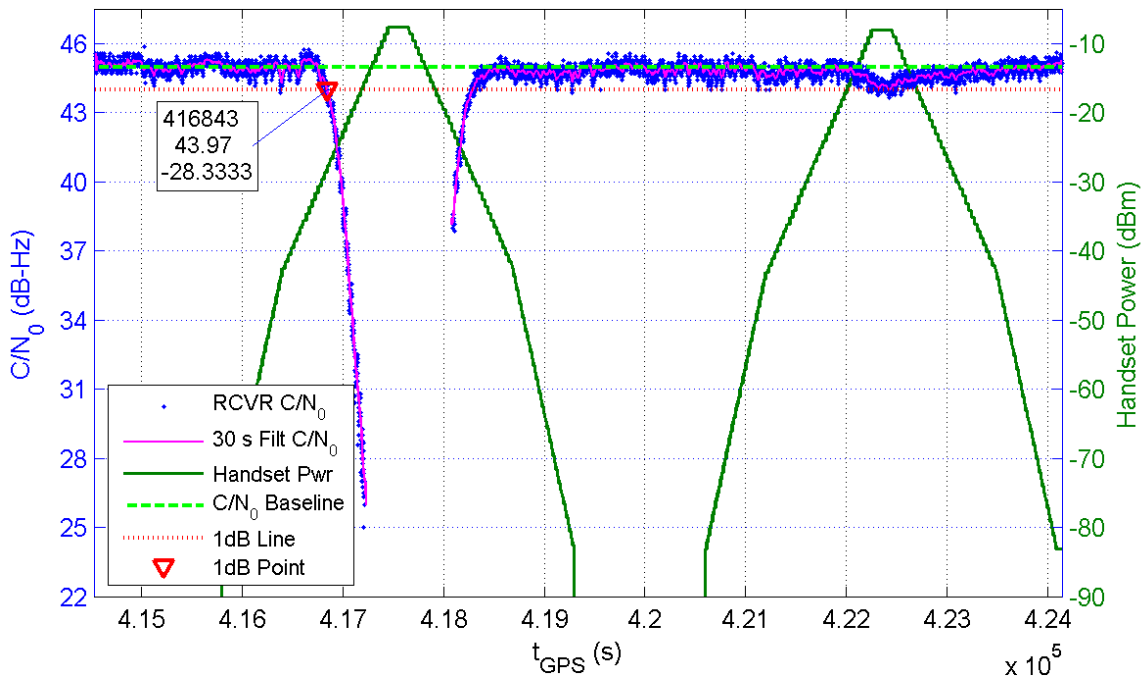
Receiver 364 Average C/N_0 for All Channels and Handset Power at Receiver for TE16/17
