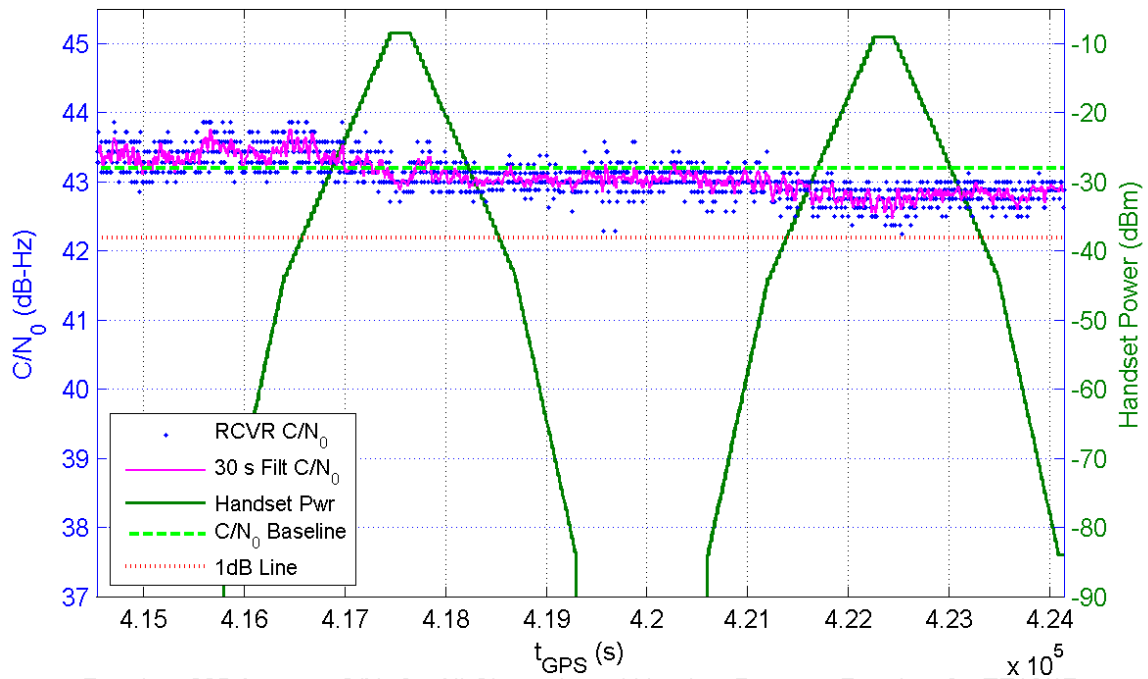
Receiver 205 Average C/N_0 for All Channels and Handset Power at Receiver for TE16/17
