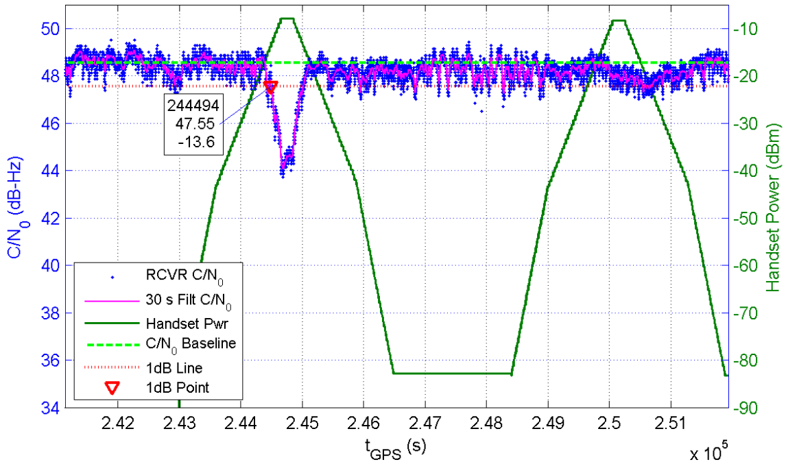
Receiver 346 Average C/N_0 for All Channels and Handset Power at Receiver for TE7/8
