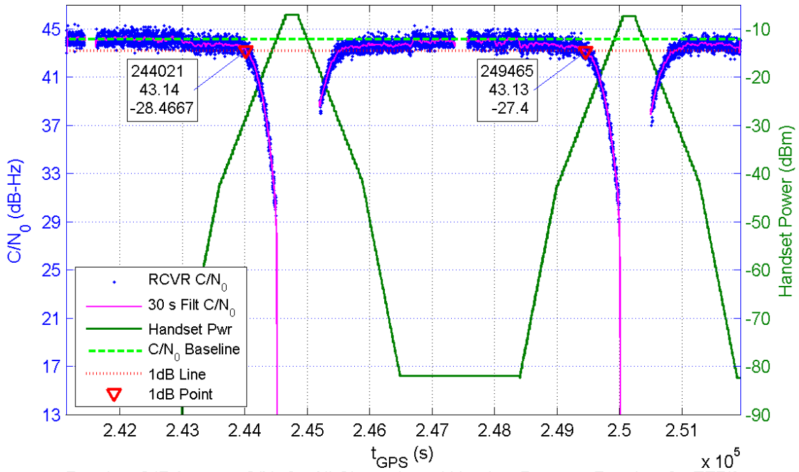
Receiver 247 Average C/N_0 for All Channels and Handset Power at Receiver for TE7/8
