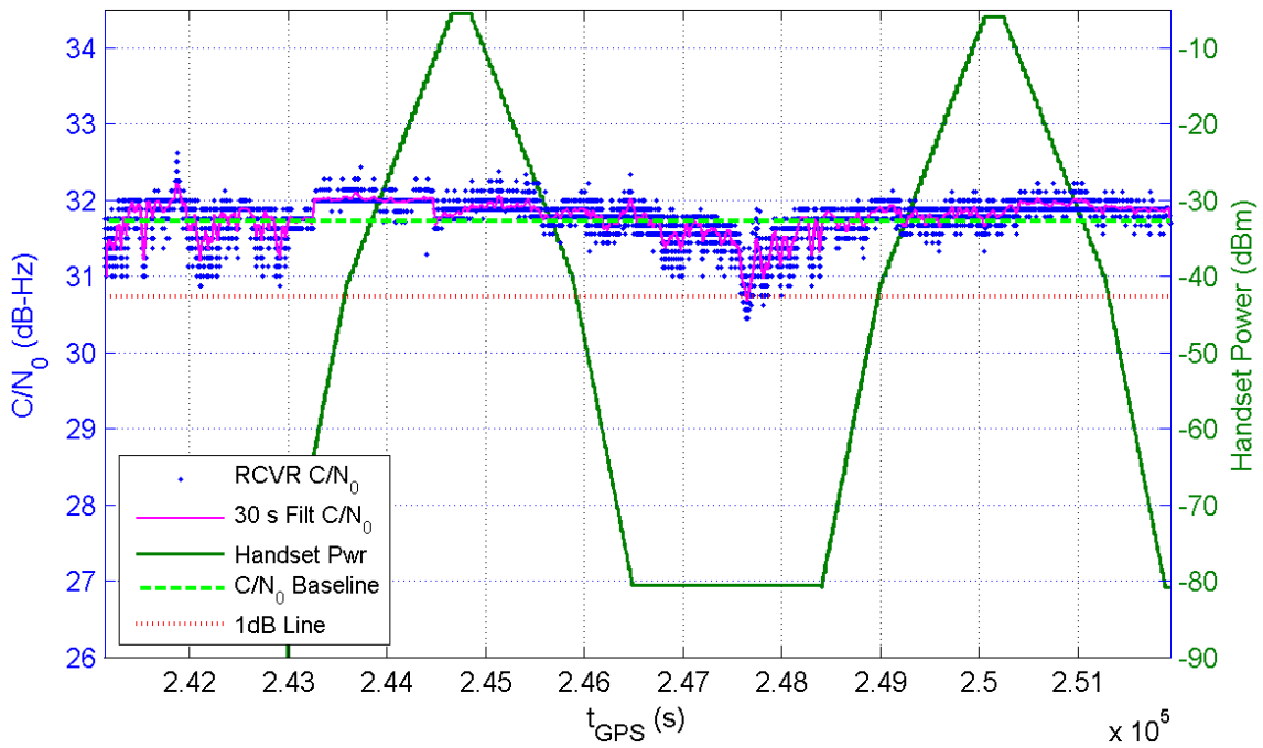
Receiver 322 Average C/N_0 for All Channels and Handset Power at Receiver for TE7/8
