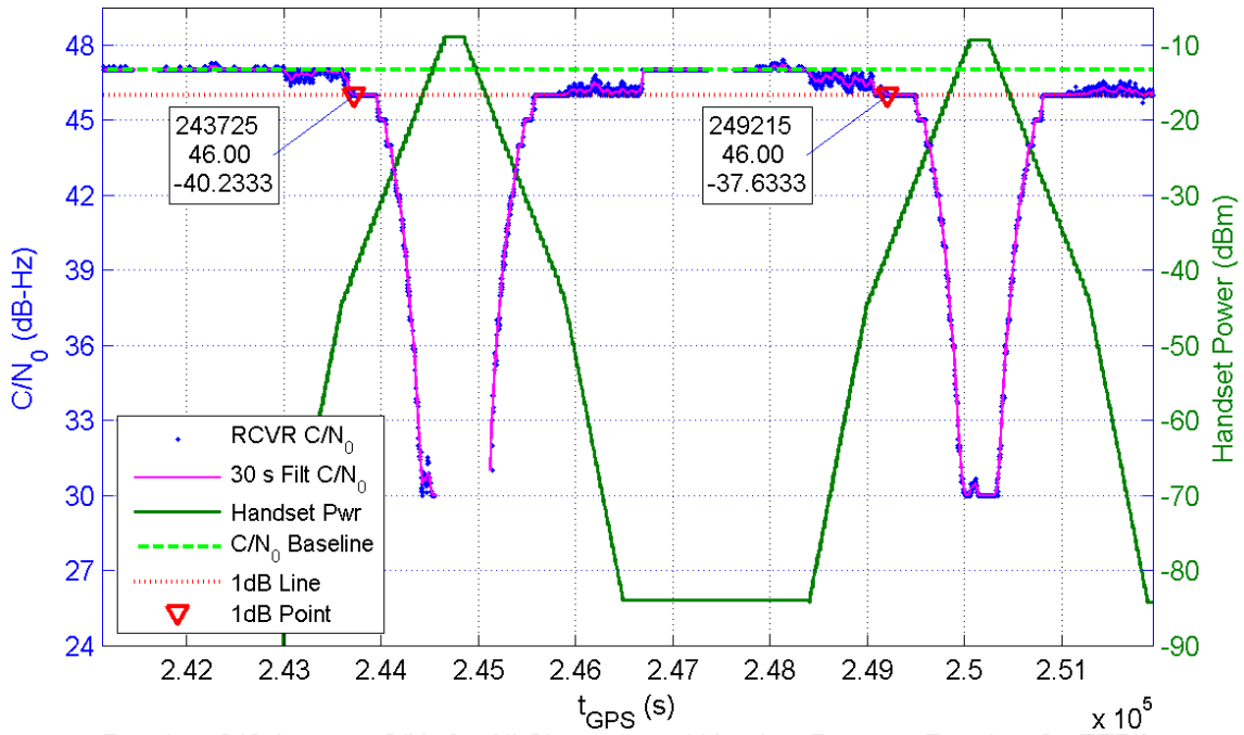
Receiver 249 Average C/N_0 for All Channels and Handset Power at Receiver for TE7/8
