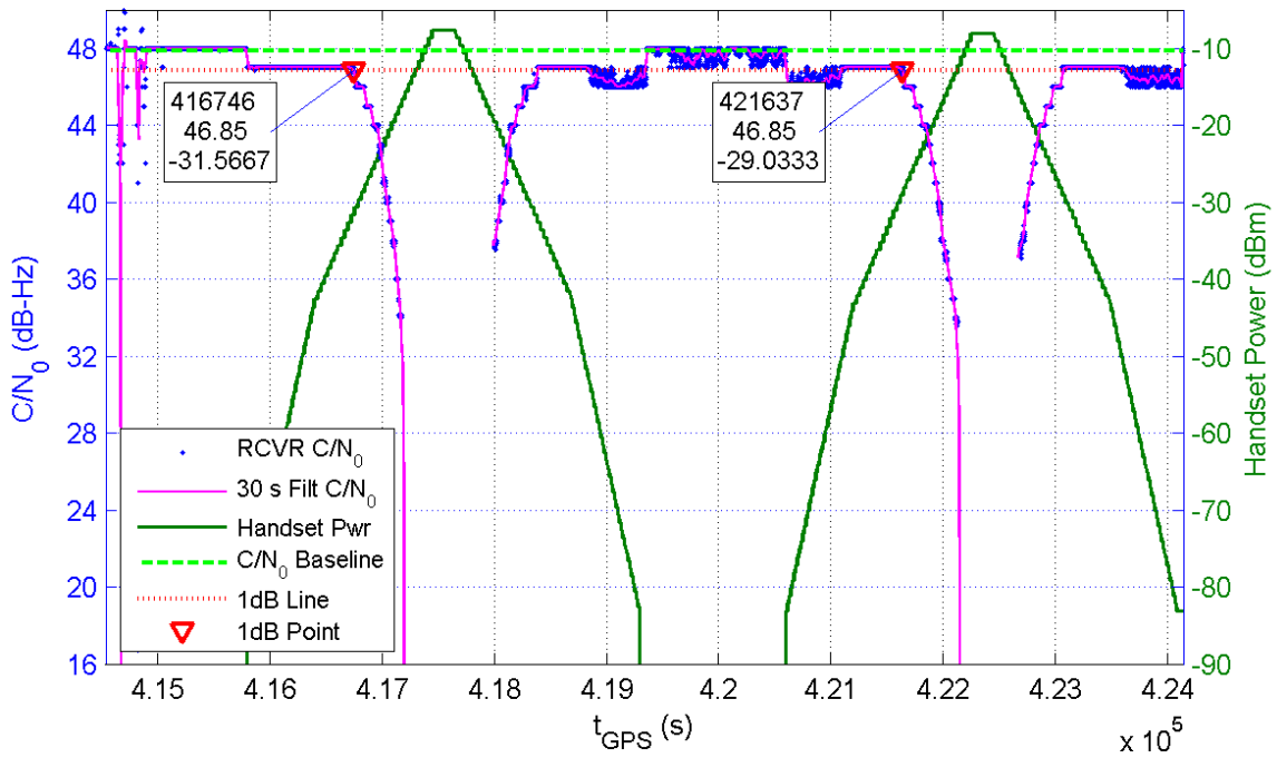
Receiver 304 Average C/N_0 for All Channels and Handset Power at Receiver for TE16/17
