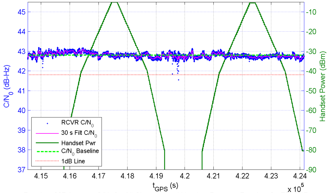
Receiver 327 Average C/N_0 for All Channels and Handset Power at Receiver for TE16/17
