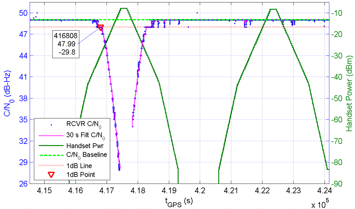
Receiver 111 Average C/N_0 for All Channels and Handset Power at Receiver for TE16/17
