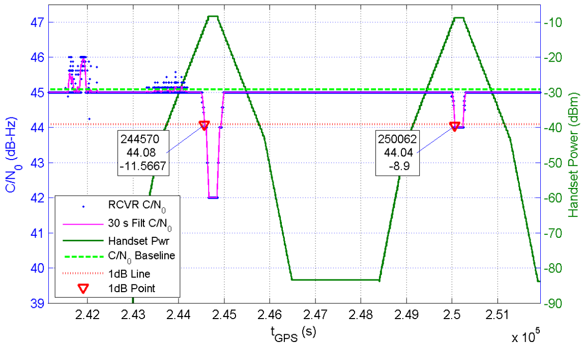
Receiver 124 Average C/N_0 for All Channels and Handset Power at Receiver for TE7/8
