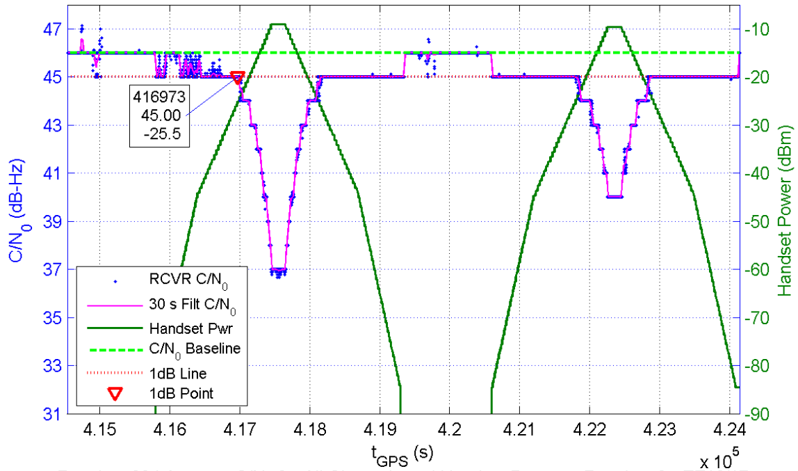
Receiver 334 Average C/N_0 for All Channels and Handset Power at Receiver for TE16/17
