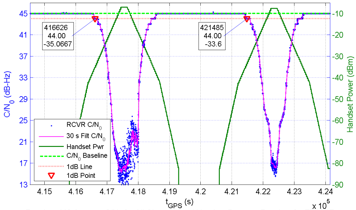
Receiver 113 Average C/N 0 for All Channels and Handset Power at Receiver for TE16/17
