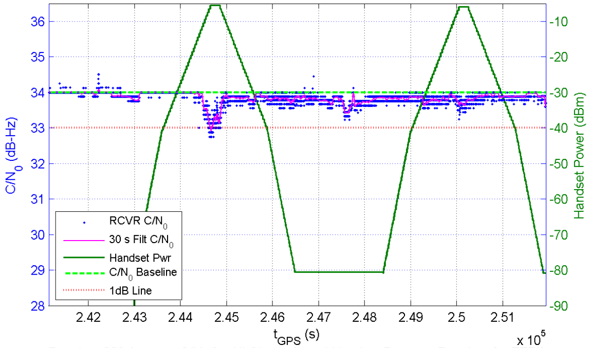
Receiver 206 Average C/N_0 for All Channels and Handset Power at Receiver for TE7/8
