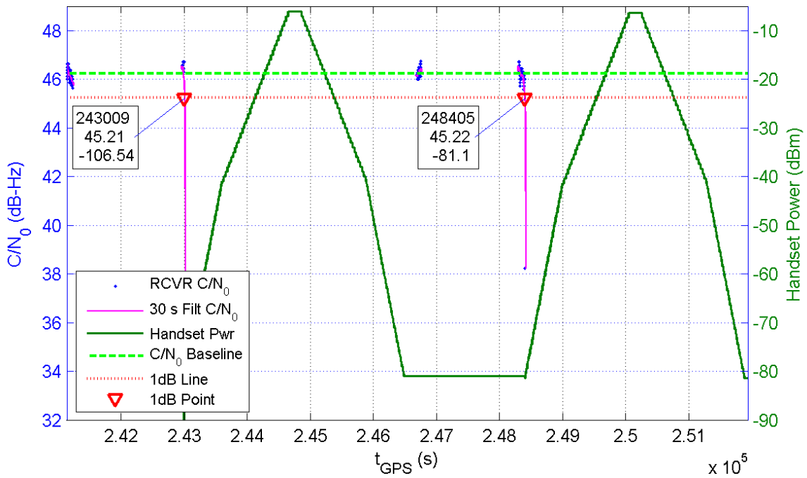
Receiver 129 Average C/N_0 for All Channels and Handset Power at Receiver for TE7/8
