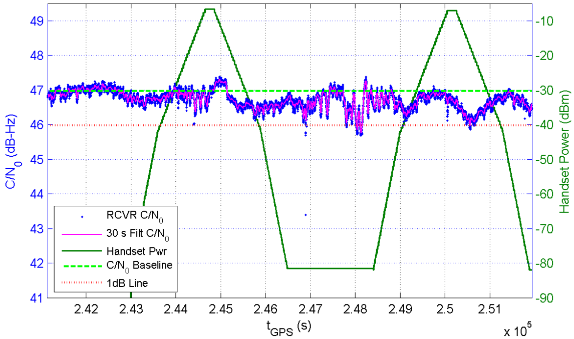
Receiver 202 Average C/N_0 for All Channels and Handset Power at Receiver for TE7/8
