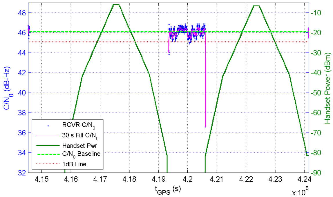
Receiver 129 Average C/N_0 for All Channels and Handset Power at Receiver for TE16/17
