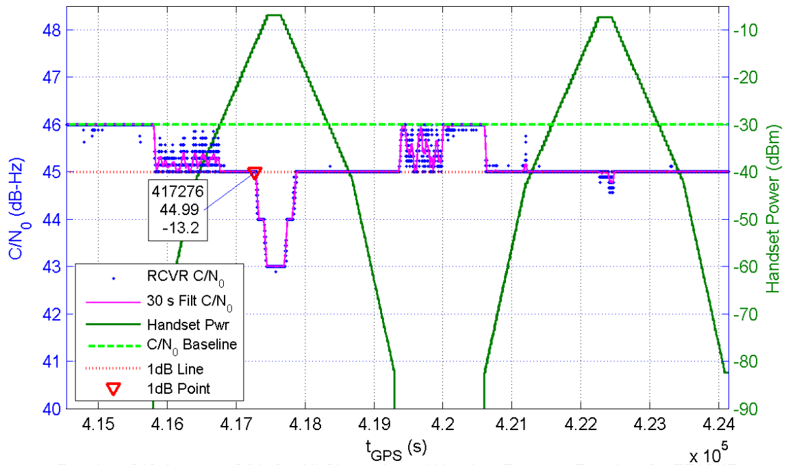
Receiver 219 Average C/N_0 for All Channels and Handset Power at Receiver for TE16/17
