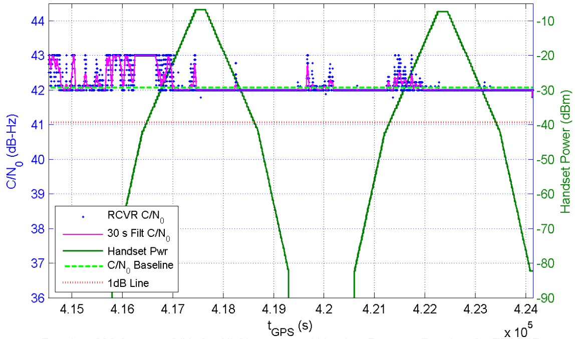
Receiver 336 Average C/N_0 for All Channels and Handset Power at Receiver for TE16/17
