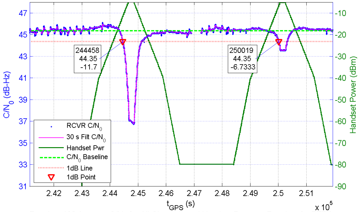
Receiver 132 Average C/N_0 for All Channels and Handset Power at Receiver for TE7/8
