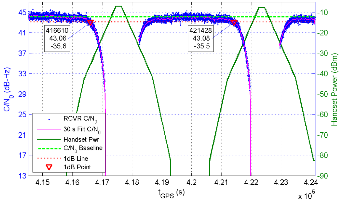
Receiver 246 Average C/N_0 for All Channels and Handset Power at Receiver for TE16/17
