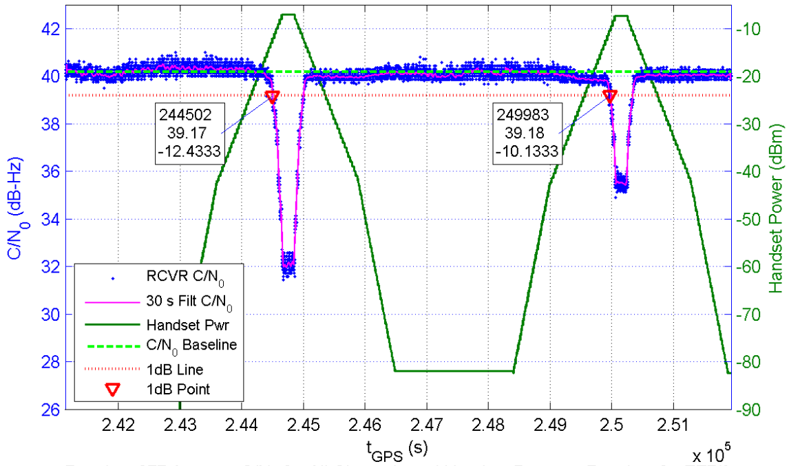
Receiver 377 Average C/N_0 for All Channels and Handset Power at Receiver for TE7/8
