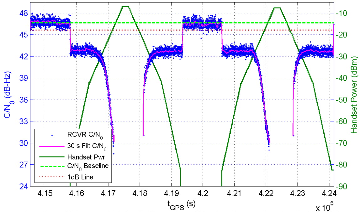
Receiver 248 Average C/N_0 for All Channels and Handset Power at Receiver for TE16/17
