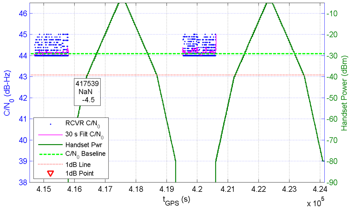
Receiver 357 Average C/N_0 for All Channels and Handset Power at Receiver for TE16/17
