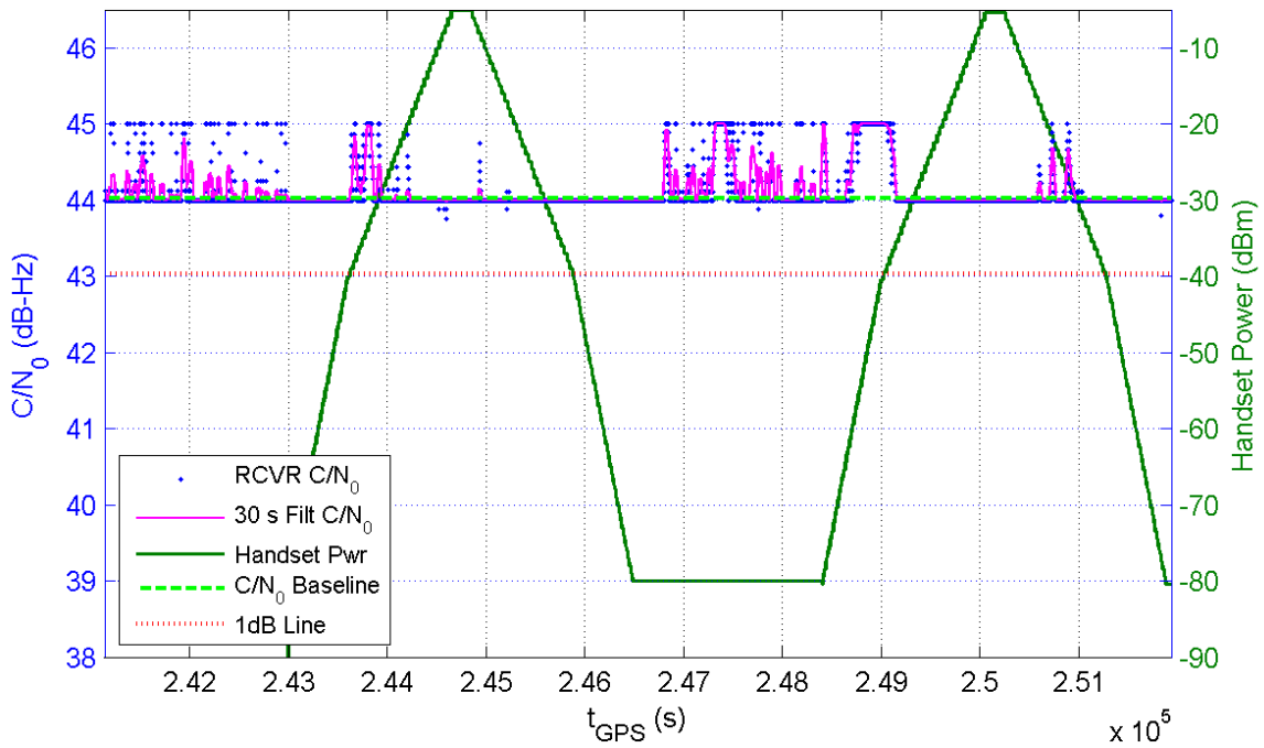
Receiver 338 Average C/N_0 for All Channels and Handset Power at Receiver for TE7/8
