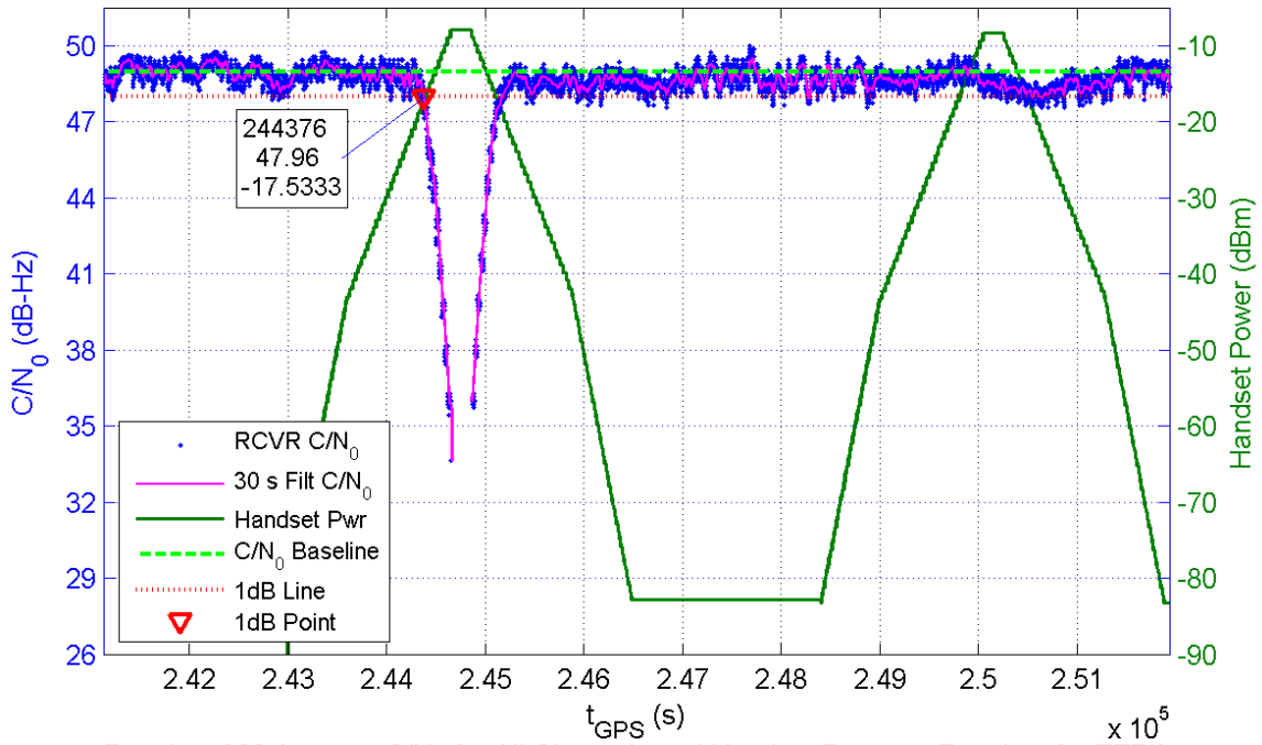
Receiver 322 Average C/N_0 for All Channels and Handset Power at Receiver for TE7/8
