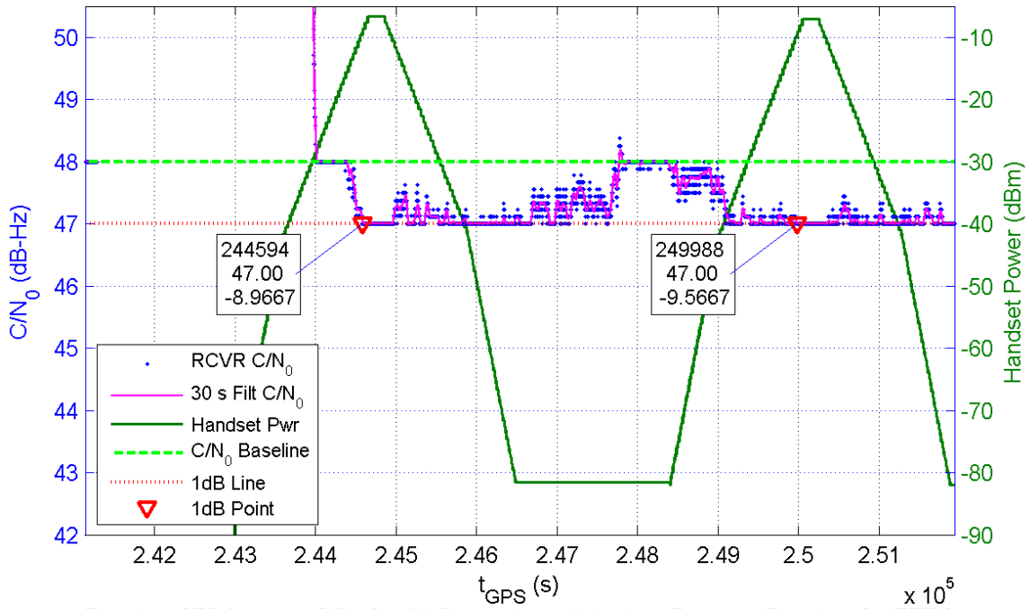
Receiver 370 Average C/N_0 for All Channels and Handset Power at Receiver for TE7/8
