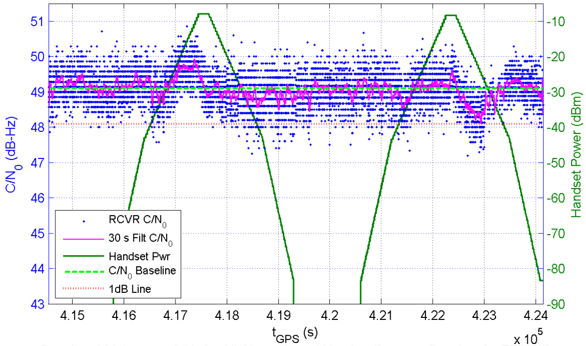
Receiver 364 Average C/N_0 for All Channels and Handset Power at Receiver for TE16/17
