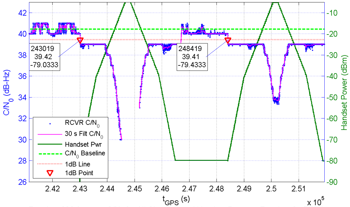
Receiver 396 Average C/N_0 for All Channels and Handset Power at Receiver for TE7/8
