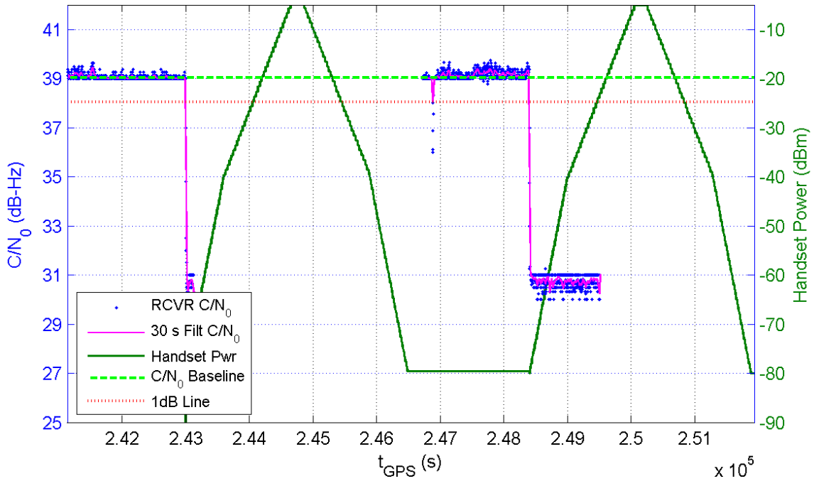
Receiver 328 Average C/N_0 for All Channels and Handset Power at Receiver for TE7/8
