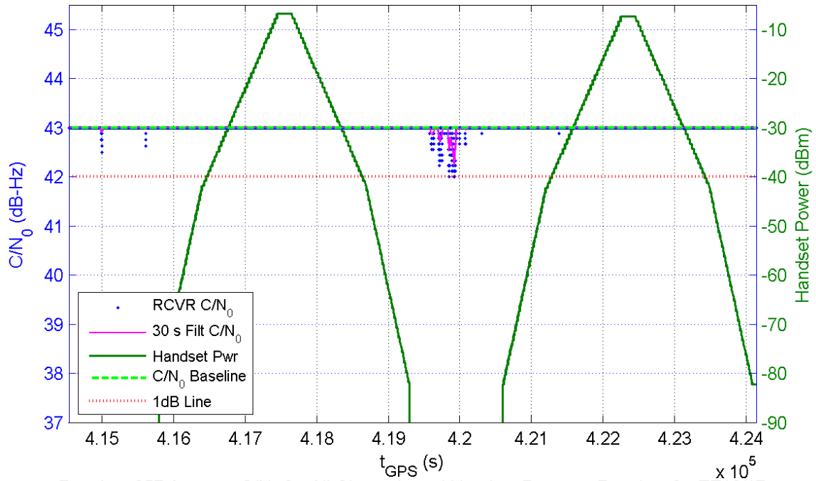
Receiver 357 Average C/N_0 for All Channels and Handset Power at Receiver for TE16/17
