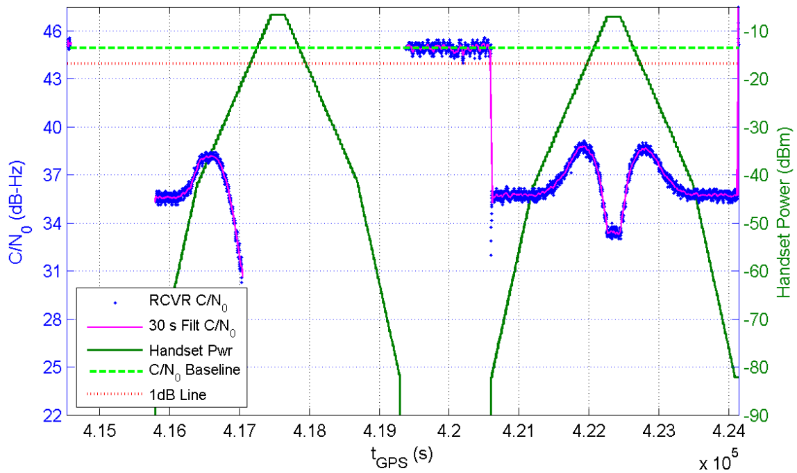
Receiver 104 Average C/N_0 for All Channels and Handset Power at Receiver for TE16/17
