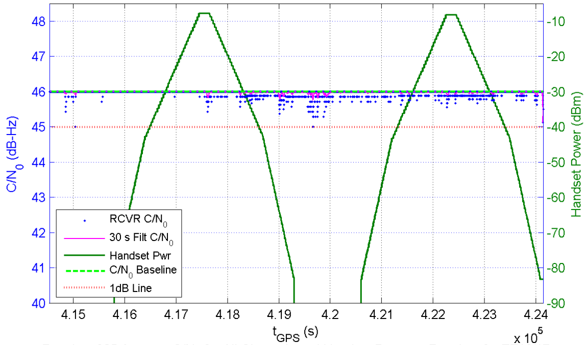
Receiver 325 Average C/N_0 for All Channels and Handset Power at Receiver for TE16/17
