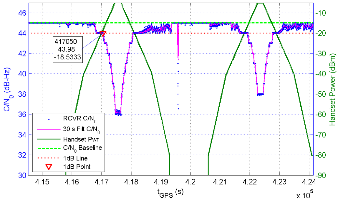
Receiver 336 Average C/N_0 for All Channels and Handset Power at Receiver for TE16/17
