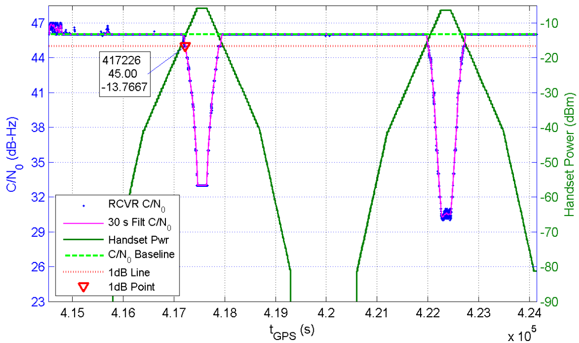
Receiver 205 Average C/N_0 for All Channels and Handset Power at Receiver for TE16/17
