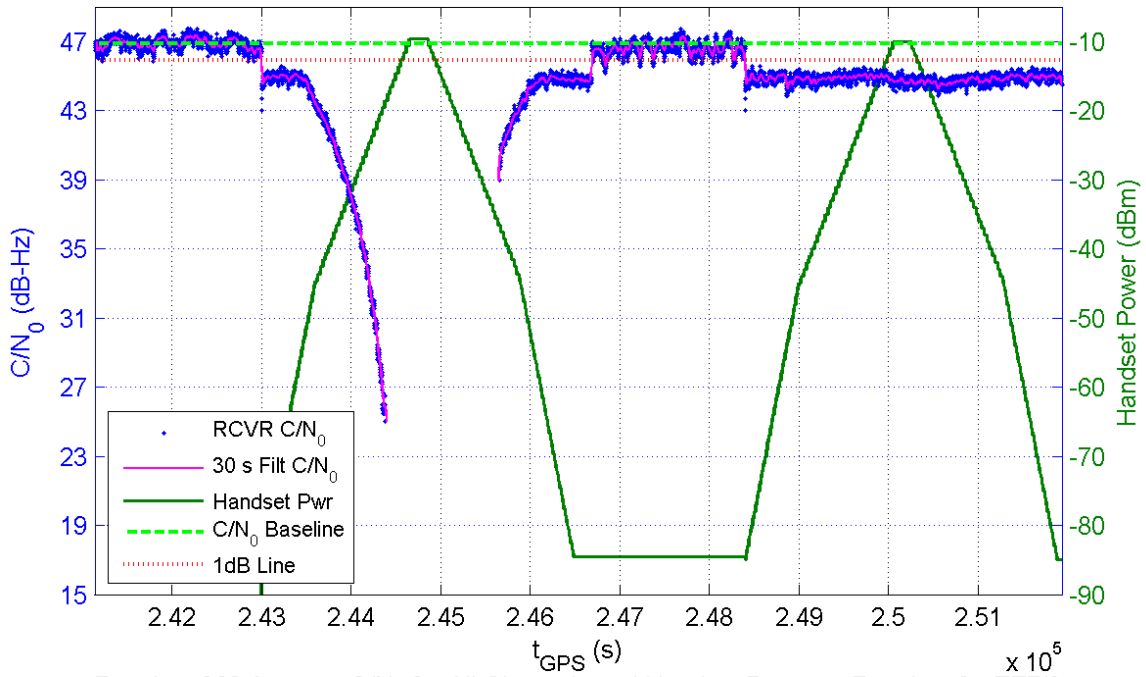
Receiver 360 Average C/N_0 for All Channels and Handset Power at Receiver for TE7/8
