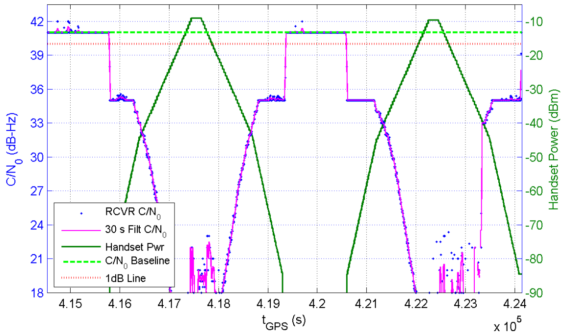
Receiver 347 Average C/N_0 for All Channels and Handset Power at Receiver for TE16/17
