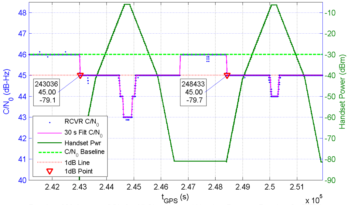
Receiver 333 Average C/N_0 for All Channels and Handset Power at Receiver for TE7/8
