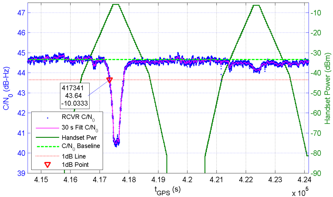
Receiver 310 Average C/N_0 for All Channels and Handset Power at Receiver for TE16/17
