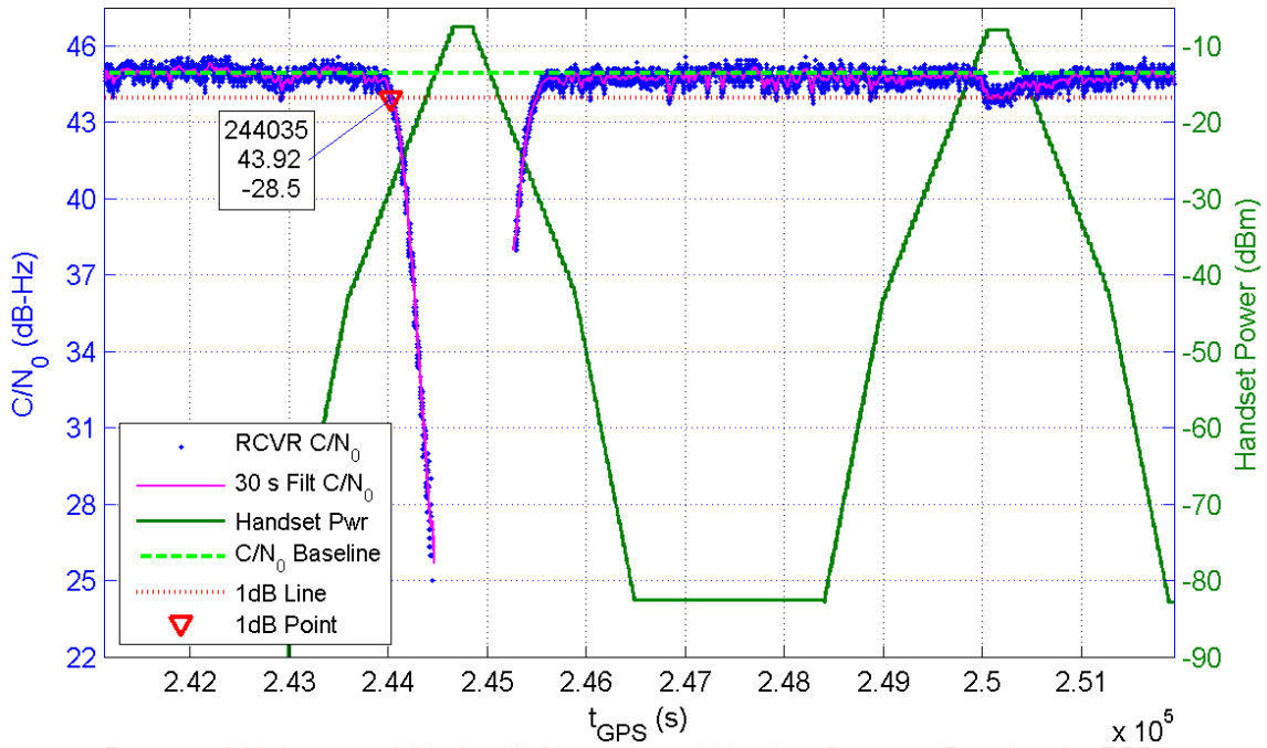
Receiver 366 Average C/N_0 for All Channels and Handset Power at Receiver for TE7/8
