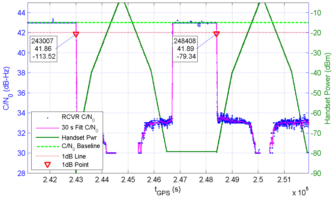
Receiver 366 Average C/N_0 for All Channels and Handset Power at Receiver for TE7/8
