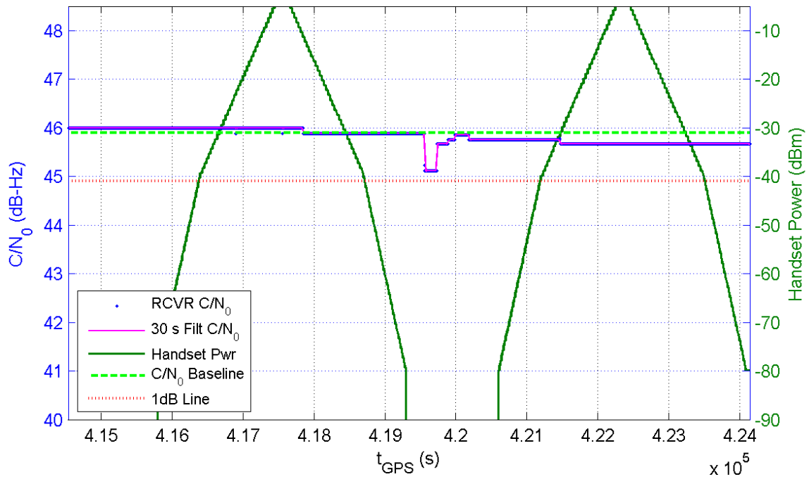
Receiver 392 Average C/N_0 for All Channels and Handset Power at Receiver for TE16/17
