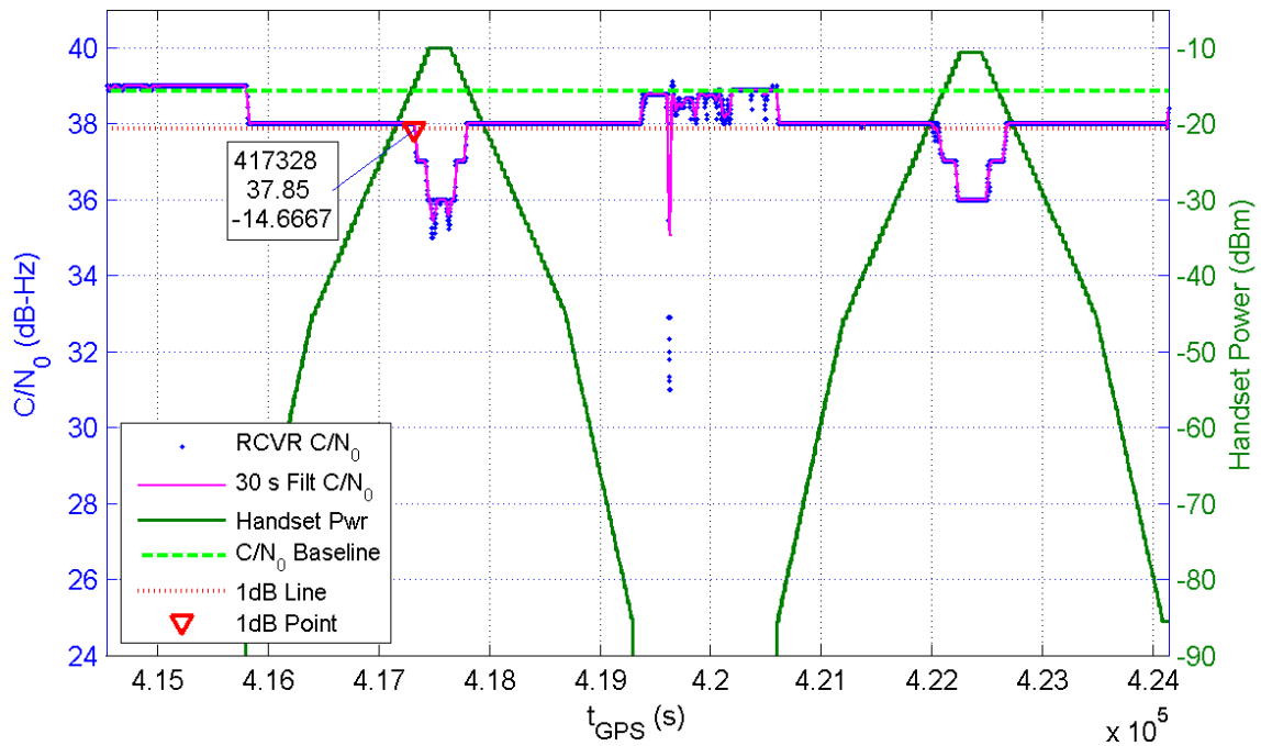
Receiver 208 Average C/N_0 for All Channels and Handset Power at Receiver for TE16/17
