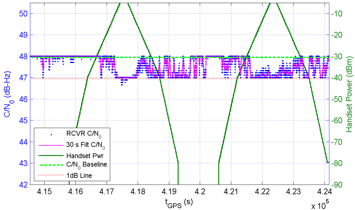
Receiver 119 Average C/N_0 for All Channels and Handset Power at Receiver for TE16/17
