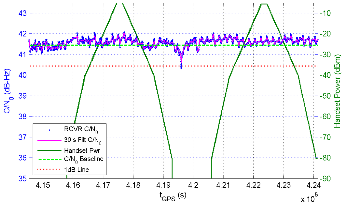
Receiver 215 Average C/N_0 for All Channels and Handset Power at Receiver for TE16/17
