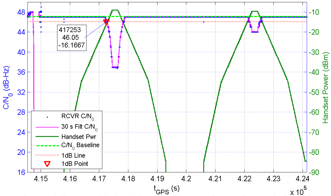
Receiver 367 Average C/N_0 for All Channels and Handset Power at Receiver for TE16/17
