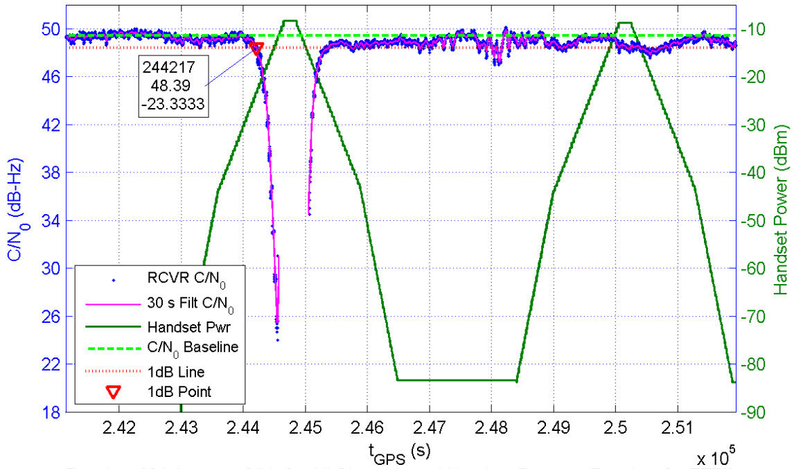
Receiver 331 Average C/N_0 for All Channels and Handset Power at Receiver for TE7/8
