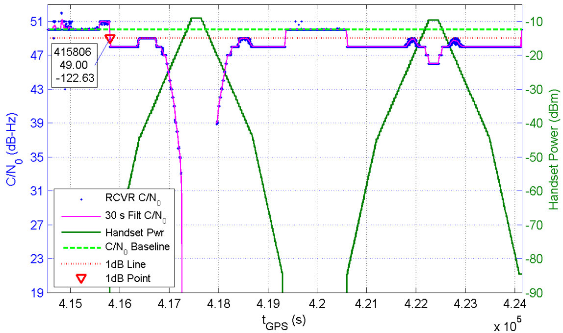
Receiver 384 Average C/N_0 for All Channels and Handset Power at Receiver for TE16/17
