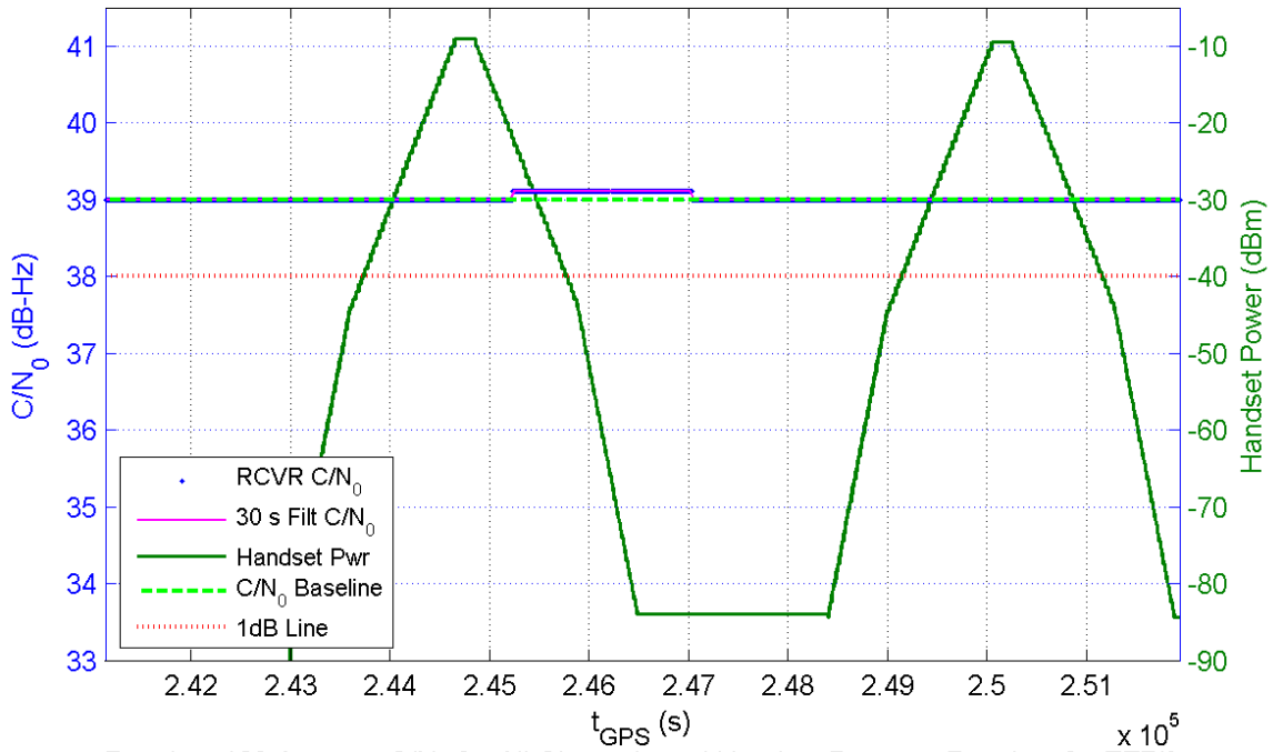
Receiver 129 Average C/N_0 for All Channels and Handset Power at Receiver for TE7/8
