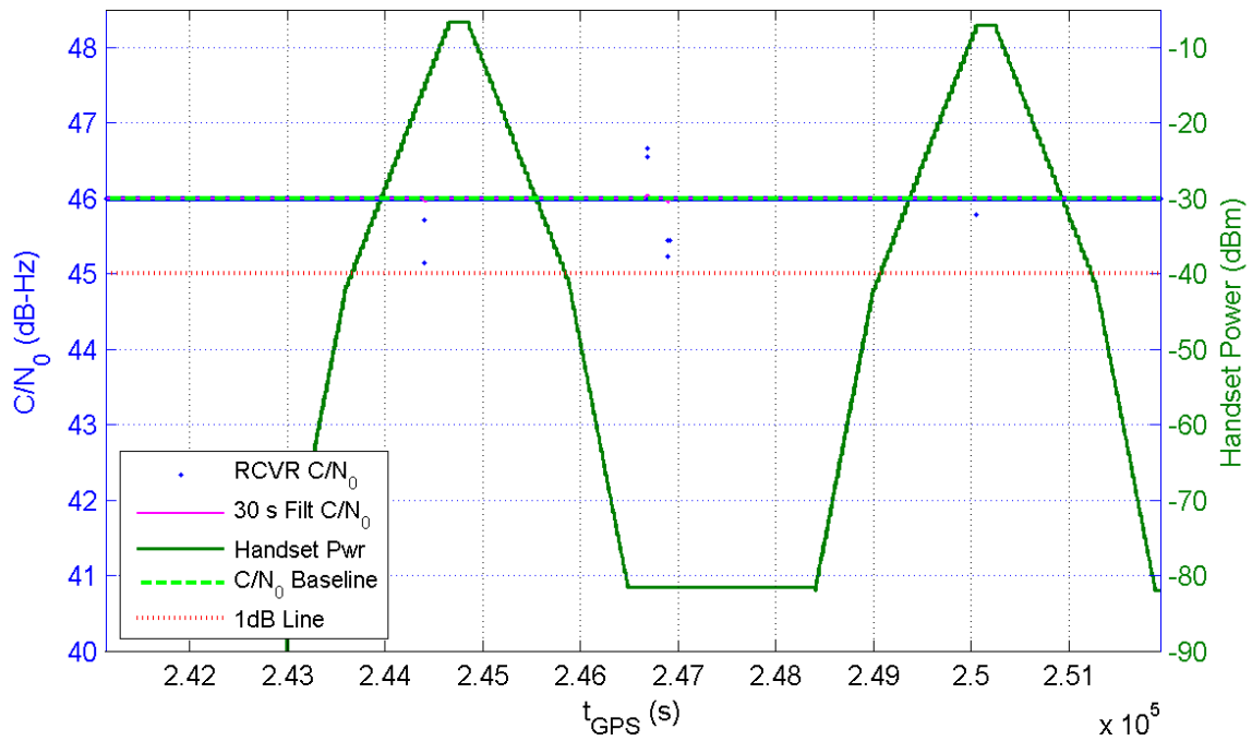
Receiver 114 Average C/N_0 for All Channels and Handset Power at Receiver for TE7/8
