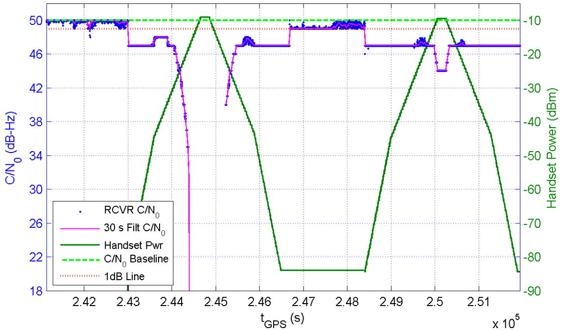
Receiver 348 Average C/N_0 for All Channels and Handset Power at Receiver for TE7/8
