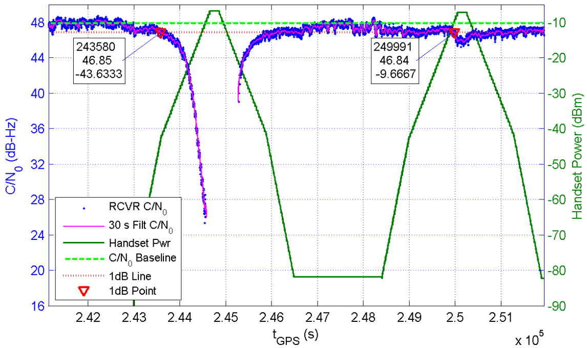
Receiver 370 Average C/N_0 for All Channels and Handset Power at Receiver for TE7/8
