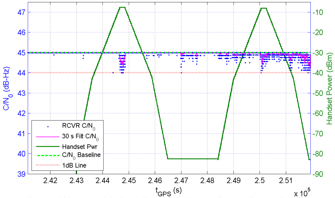
Receiver 320 Average C/N_0 for All Channels and Handset Power at Receiver for TE7/8
