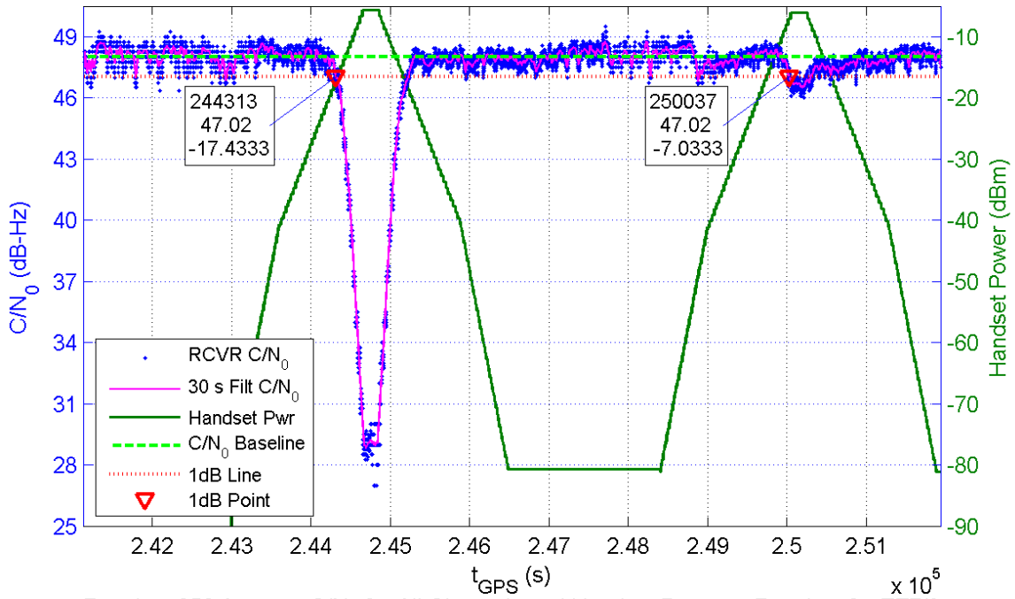
Receiver 356 Average C/N_0 for All Channels and Handset Power at Receiver for TE7/8
