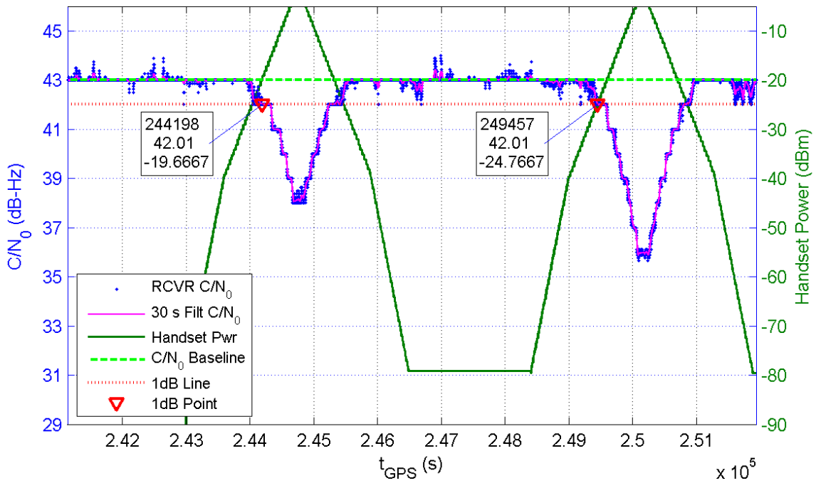
Receiver 368 Average C/N_0 for All Channels and Handset Power at Receiver for TE7/8
