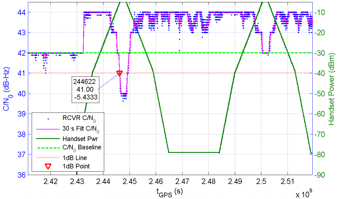
Receiver 208 Average C/N_0 for All Channels and Handset Power at Receiver for TE7/8
