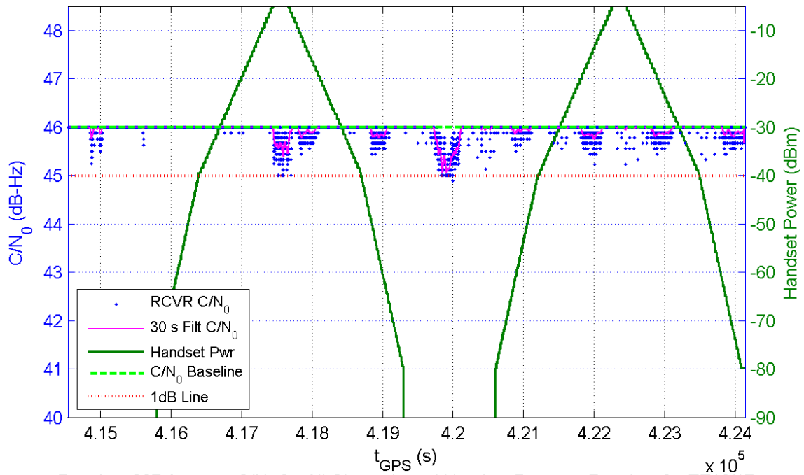
Receiver 307 Average C/N_0 for All Channels and Handset Power at Receiver for TE16/17
