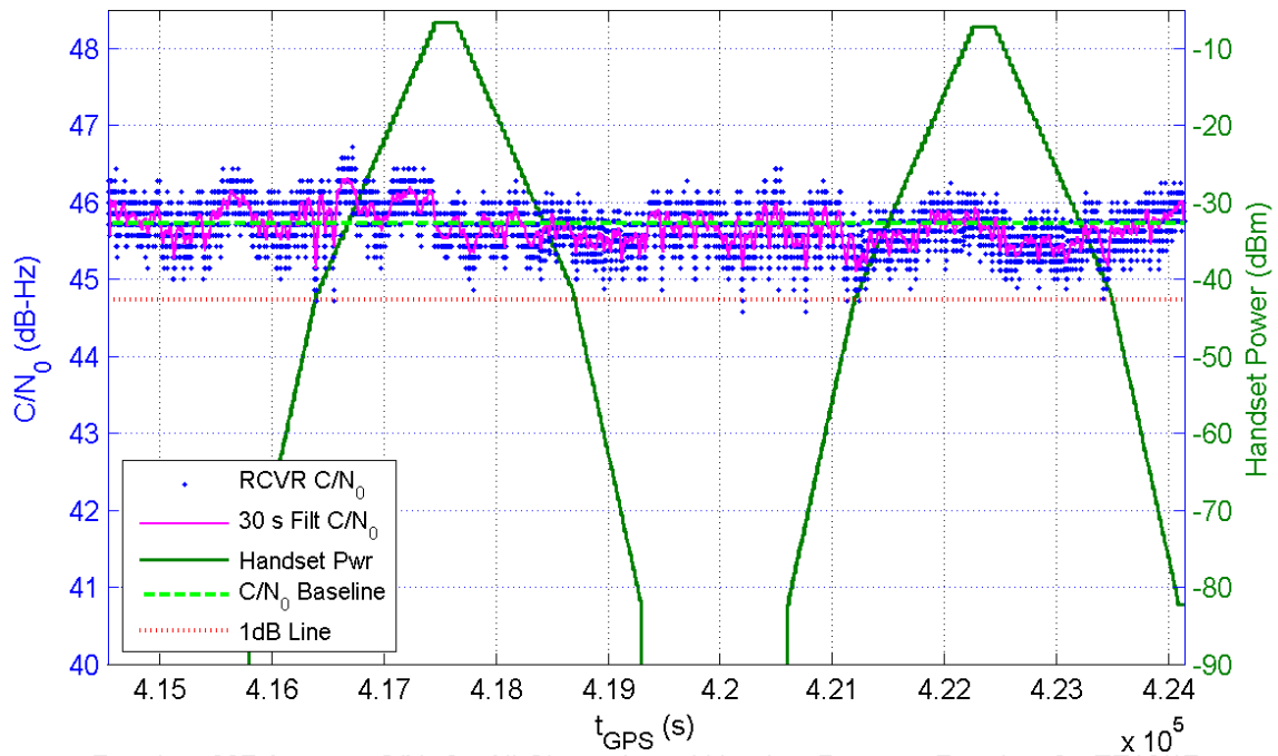
Receiver 397 Average C/N_0 for All Channels and Handset Power at Receiver for TE16/17
