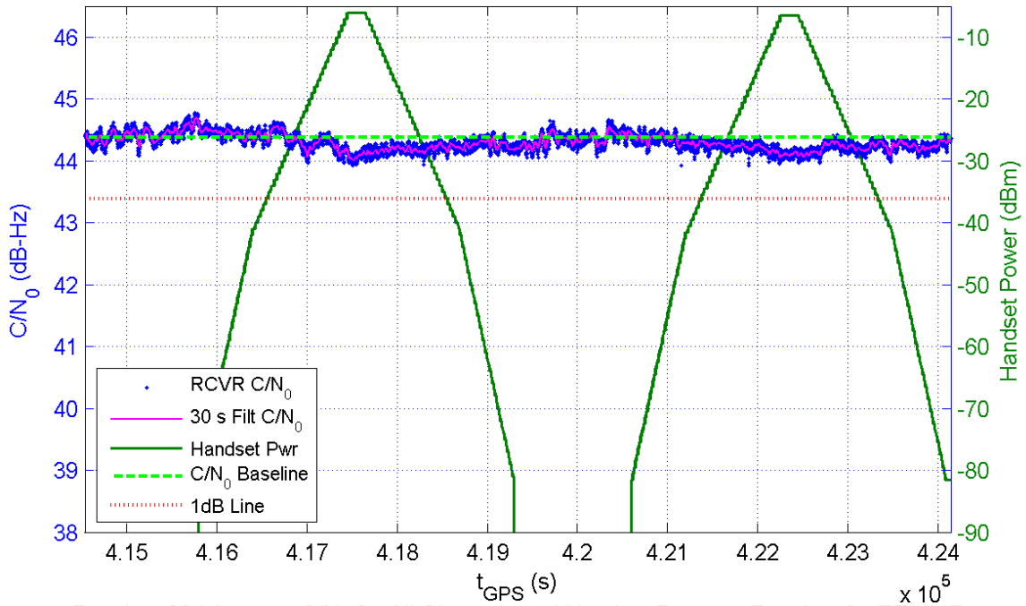
Receiver 304 Average C/N_0 for All Channels and Handset Power at Receiver for TE16/17
