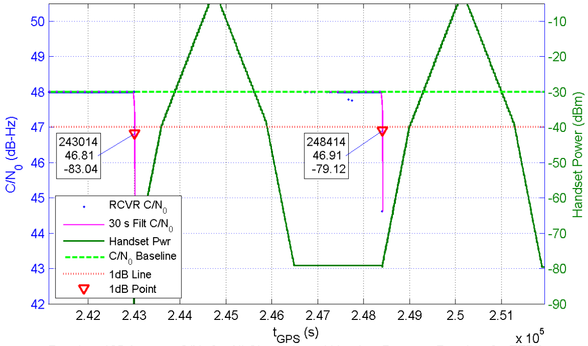
Receiver 105 Average C/N_0 for All Channels and Handset Power at Receiver for TE7/8
