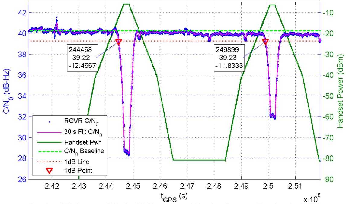
Receiver 373 Average C/N_0 for All Channels and Handset Power at Receiver for TE7/8
