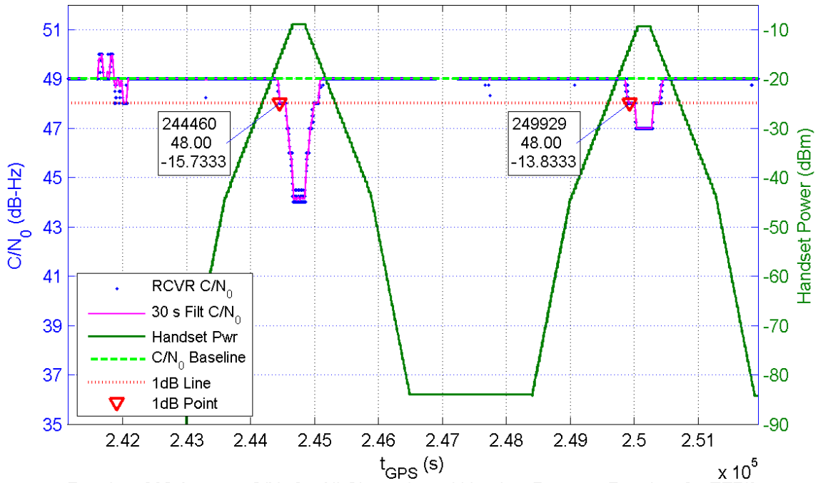
Receiver 382 Average C/N_0 for All Channels and Handset Power at Receiver for TE7/8
