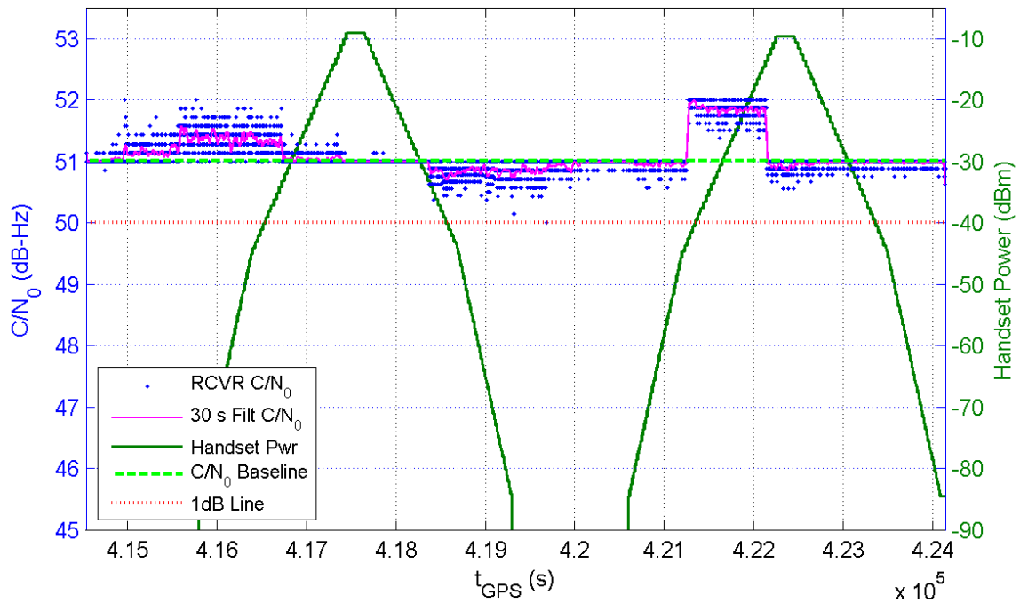
Receiver 108 Average C/N_0 for All Channels and Handset Power at Receiver for TE16/17
