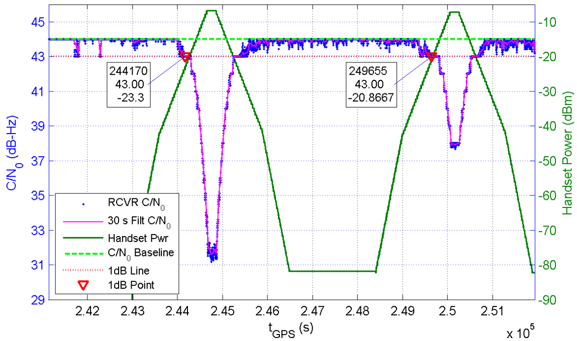
Receiver 358 Average C/N_0 for All Channels and Handset Power at Receiver for TE7/8
