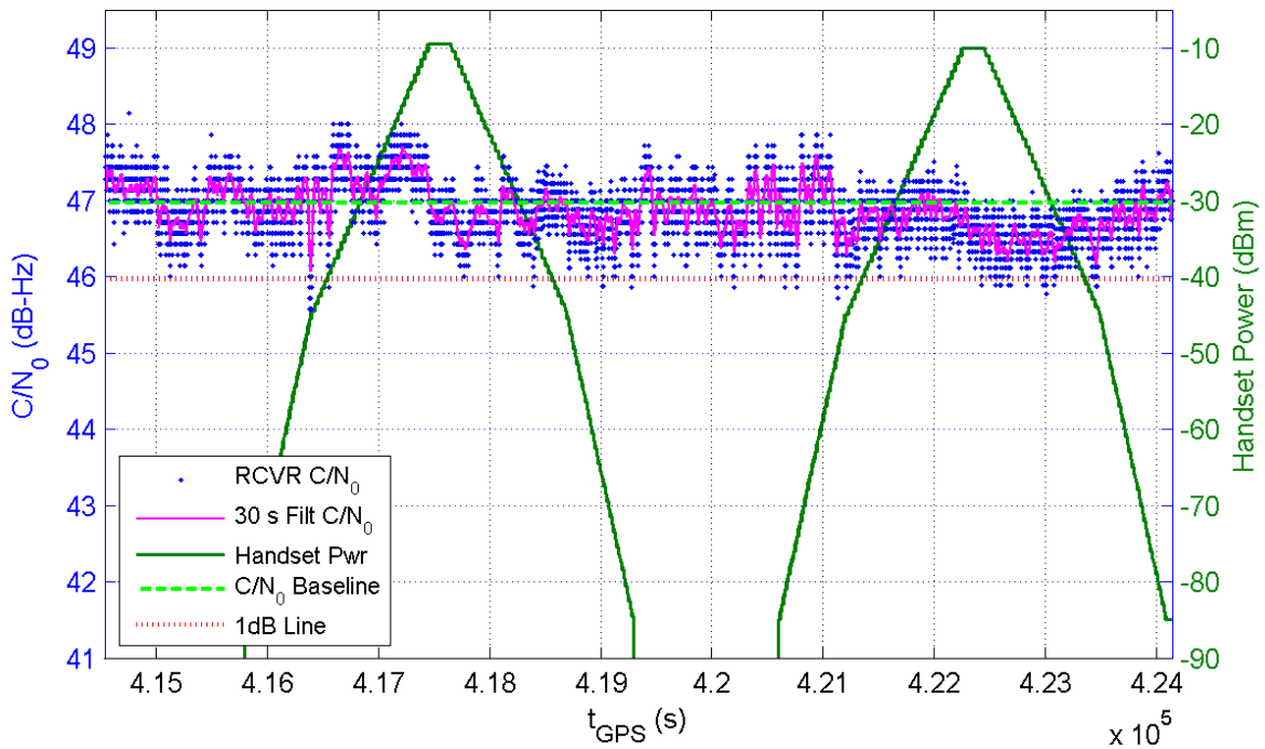
Receiver 367 Average C/N_0 for All Channels and Handset Power at Receiver for TE16/17
