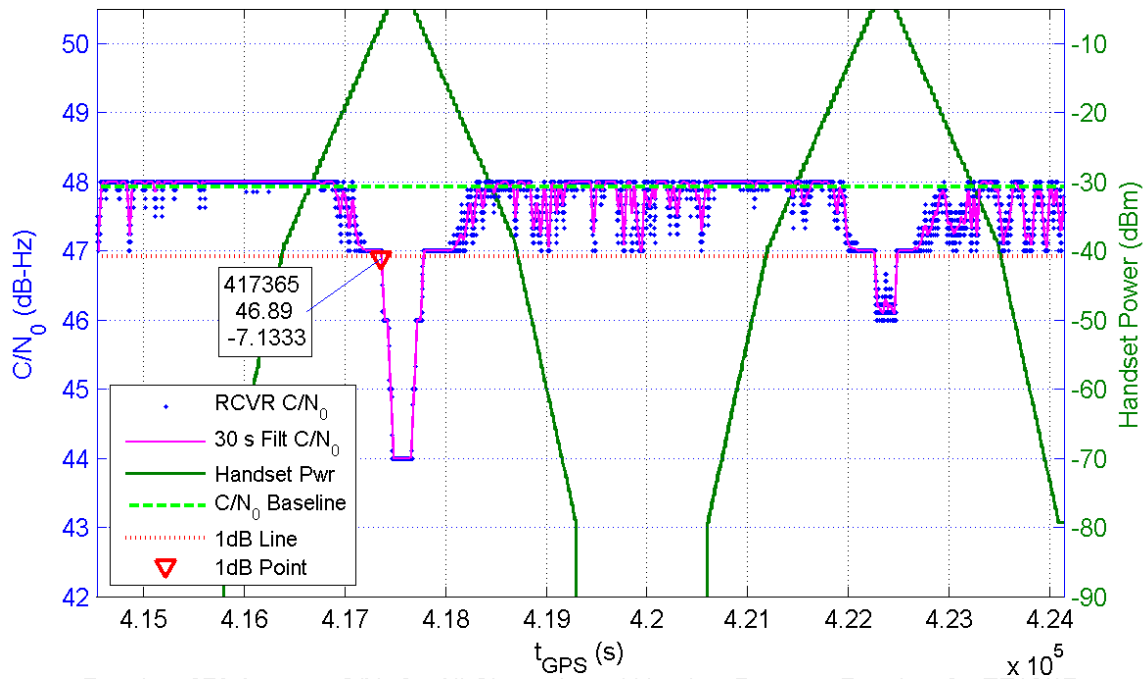
Receiver 378 Average C/N_0 for All Channels and Handset Power at Receiver for TE16/17
