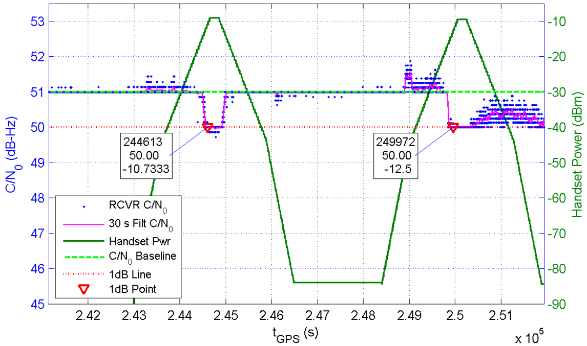
Receiver 108 Average C/N_0 for All Channels and Handset Power at Receiver for TE7/8
