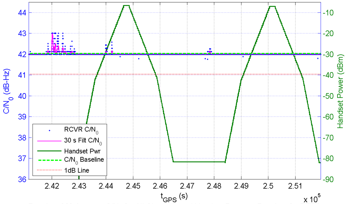
Receiver 363 Average C/N_0 for All Channels and Handset Power at Receiver for TE7/8
