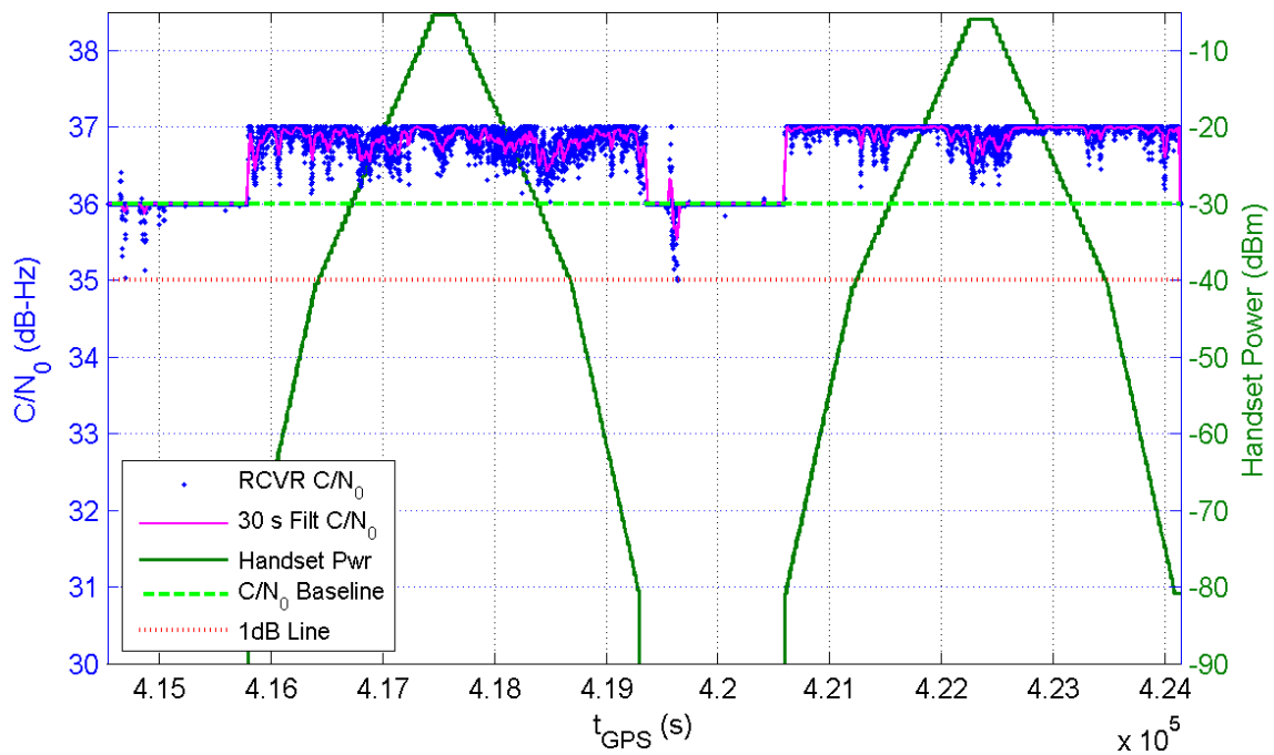
Receiver 307 Average C/N_0 for All Channels and Handset Power at Receiver for TE16/17
