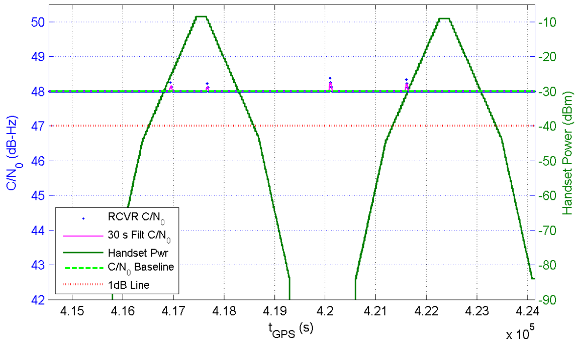
Receiver 219 Average C/N_0 for All Channels and Handset Power at Receiver for TE16/17
