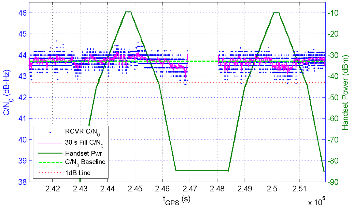
Receiver 390 Average C/N_0 for All Channels and Handset Power at Receiver for TE7/8
