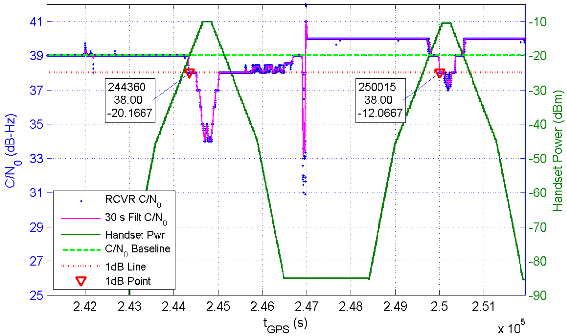
Receiver 208 Average C/N_0 for All Channels and Handset Power at Receiver for TE7/8
