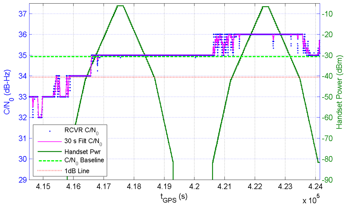
Receiver 378 Average C/N_0 for All Channels and Handset Power at Receiver for TE16/17
