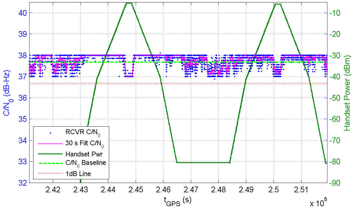
Receiver 127 Average C/N_0 for All Channels and Handset Power at Receiver for TE7/8
