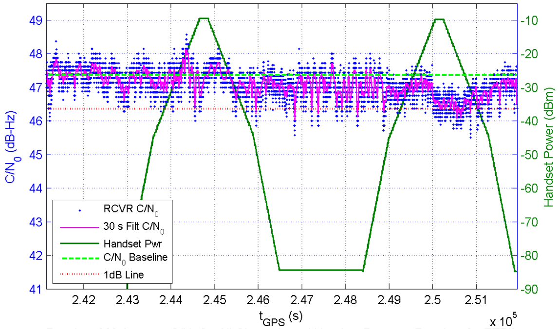
Receiver 368 Average C/N_0 for All Channels and Handset Power at Receiver for TE7/8
