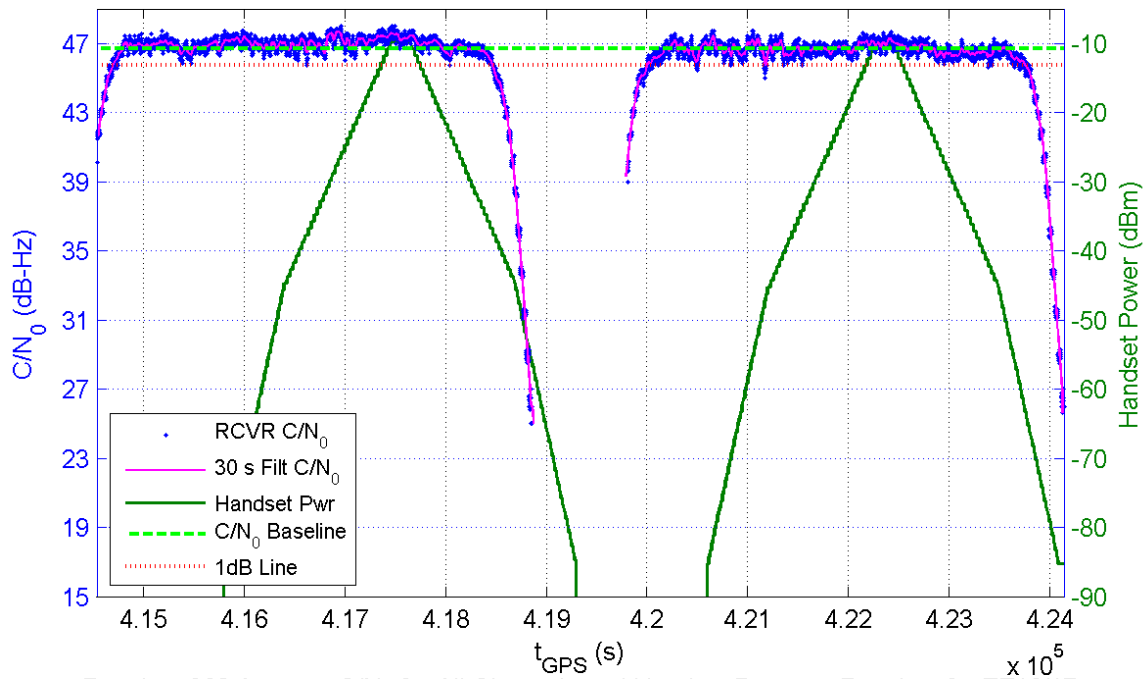
Receiver 360 Average C/N_0 for All Channels and Handset Power at Receiver for TE16/17
