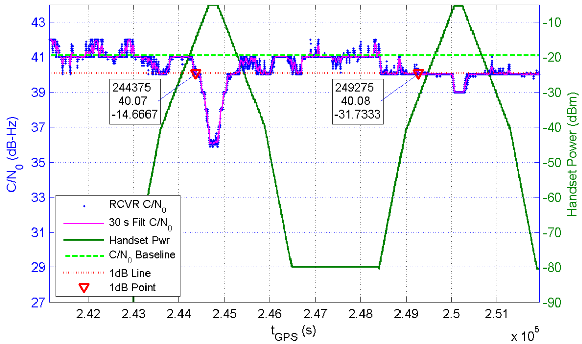
Receiver 134 Average C/N_0 for All Channels and Handset Power at Receiver for TE7/8
