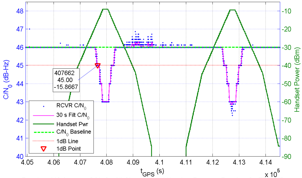
Receiver 119 Average C/N_0 for All Channels and Handset Power at Receiver for TE14/15
