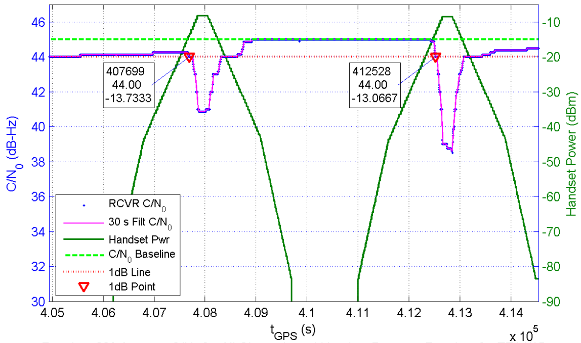
Receiver 208 Average C/N 0 for All Channels and Handset Power at Receiver for TE14/15
