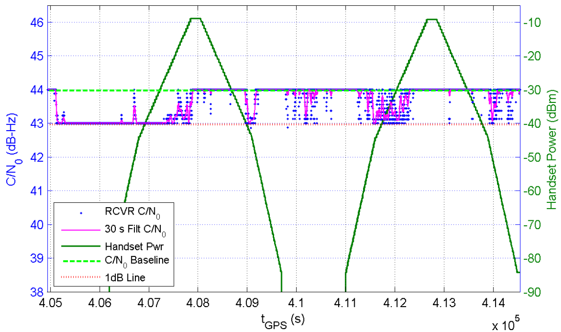
Receiver 308 Average C/N_0 for All Channels and Handset Power at Receiver for TE14/15
