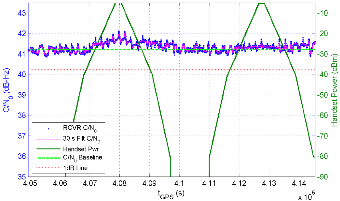
Receiver 215 Average C/N_0 for All Channels and Handset Power at Receiver for TE14/15
