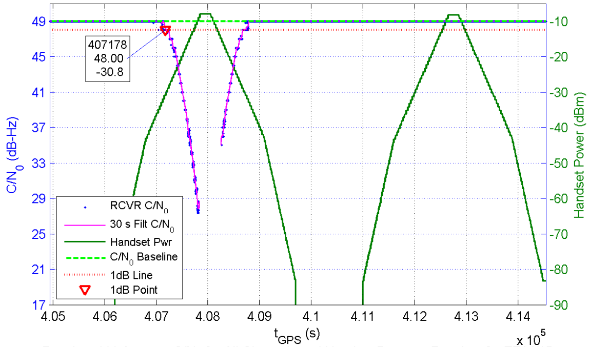
Receiver 111 Average C/N 0 for All Channels and Handset Power at Receiver for TE14/15
