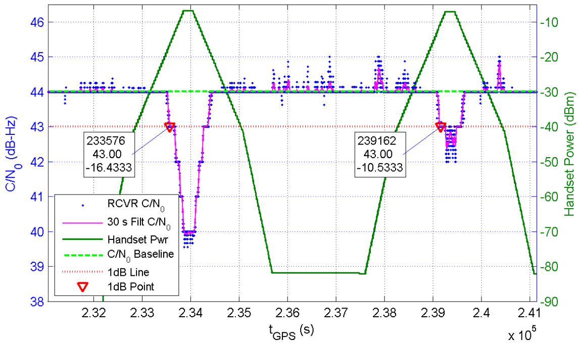
Receiver 249 Average C/N_0 for All Channels and Handset Power at Receiver for TE5/6
