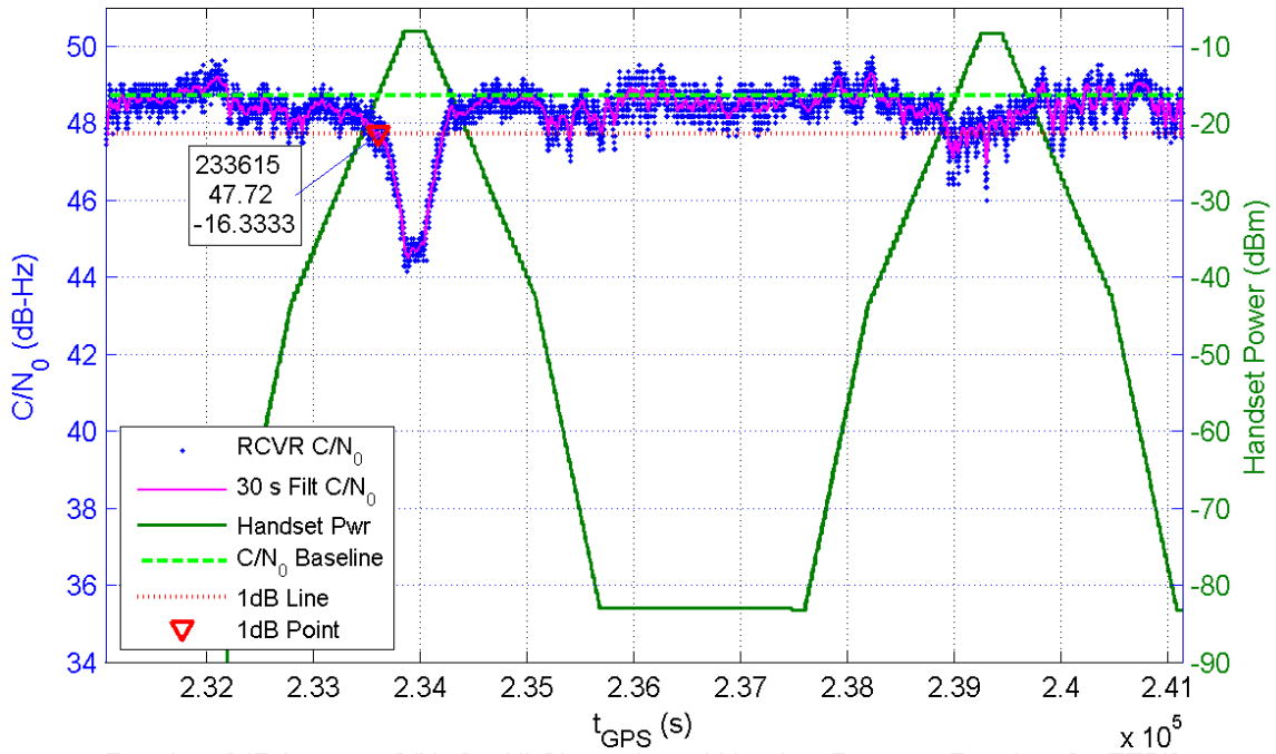
Receiver 347 Average C/N_0 for All Channels and Handset Power at Receiver for TE5/6
