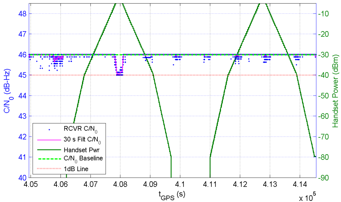
Receiver 306 Average C/N_0 for All Channels and Handset Power at Receiver for TE14/15
