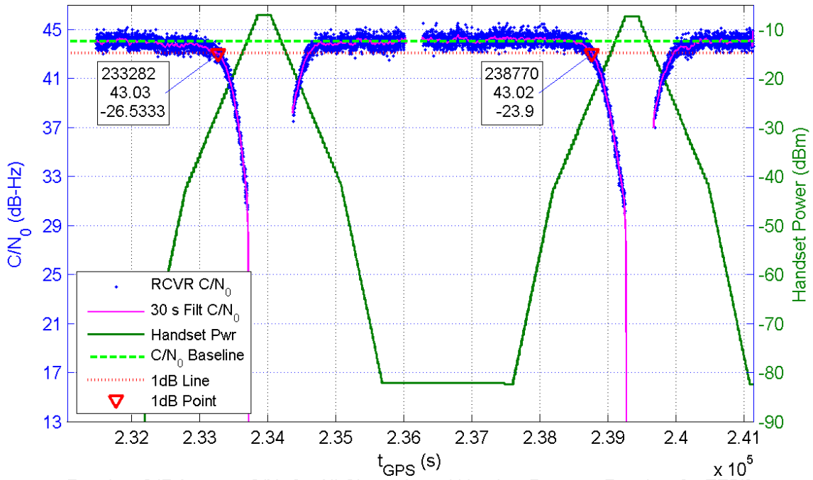
Receiver 247 Average C/N_0 for All Channels and Handset Power at Receiver for TE5/6
