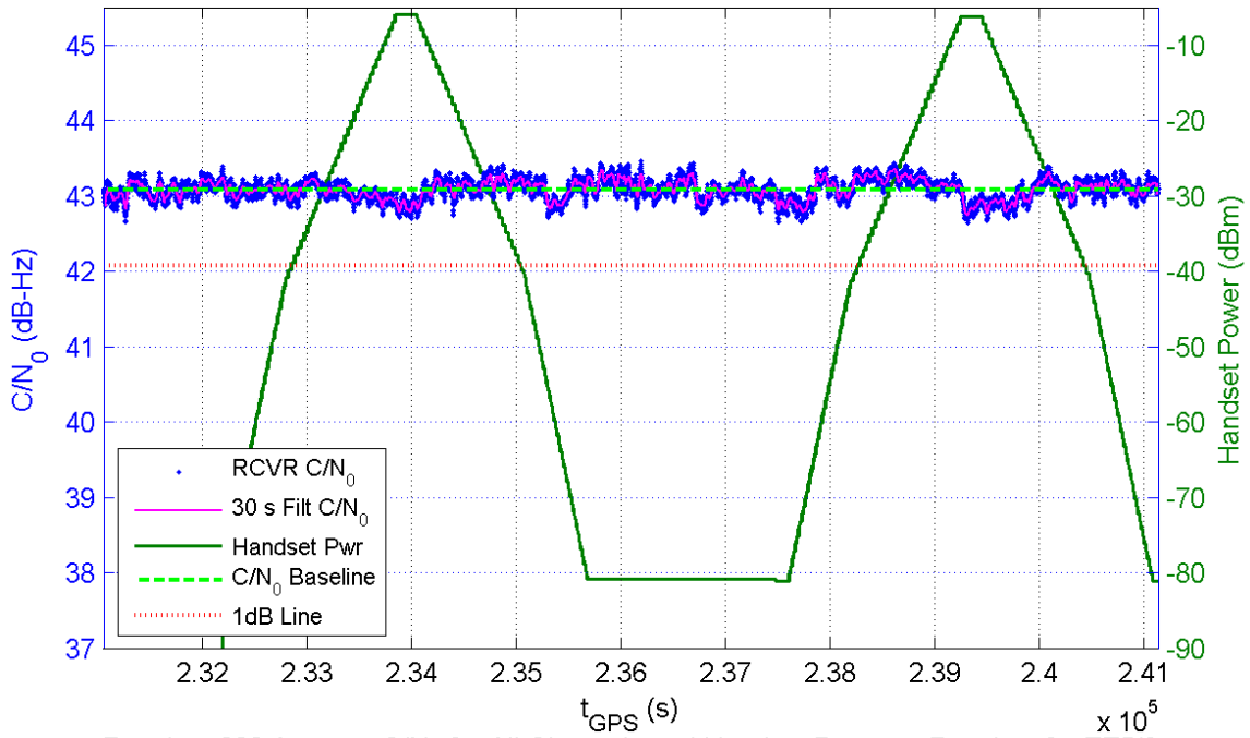
Receiver 202 Average C/N_0 for All Channels and Handset Power at Receiver for TE5/6
