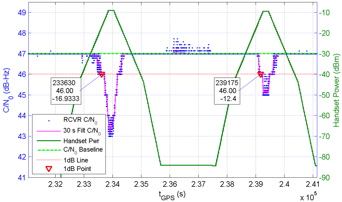
Receiver 115 Average C/N_0 for All Channels and Handset Power at Receiver for TE5/6
