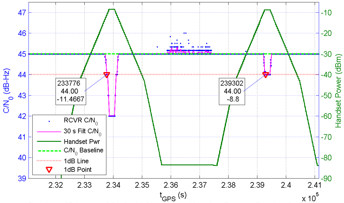
Receiver 125 Average C/N_0 for All Channels and Handset Power at Receiver for TE5/6
