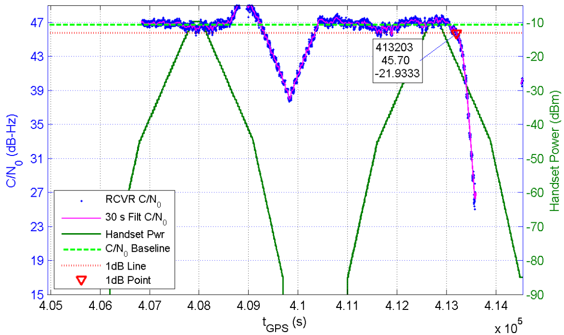
Receiver 359 Average C/N_0 for All Channels and Handset Power at Receiver for TE14/15
