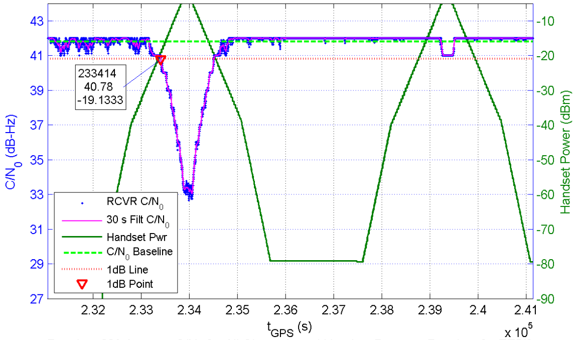
Receiver 208 Average C/N_0 for All Channels and Handset Power at Receiver for TE5/6
