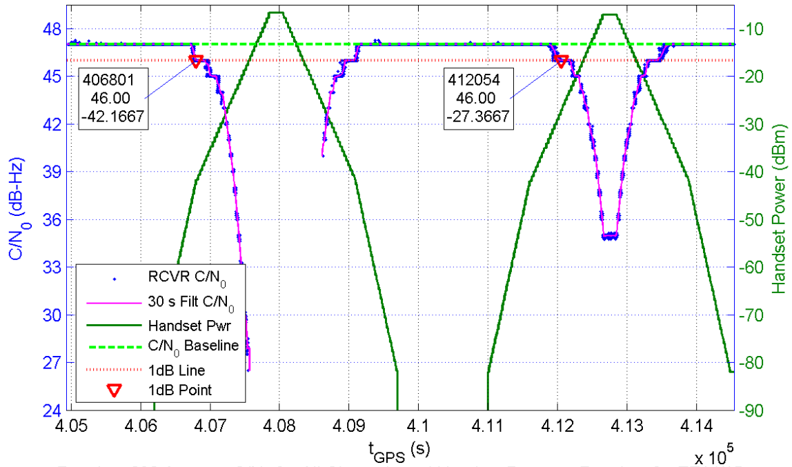
Receiver 232 Average C/N 0 for All Channels and Handset Power at Receiver for TE14/15
