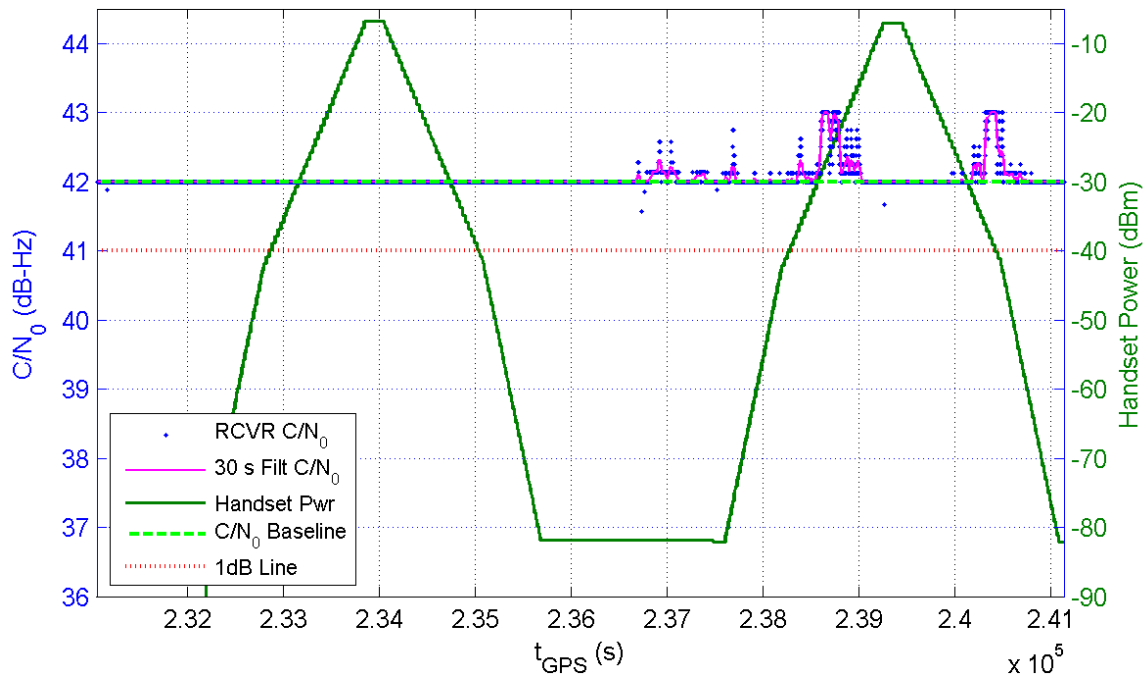
Receiver 361 Average C/N_0 for All Channels and Handset Power at Receiver for TE5/6
