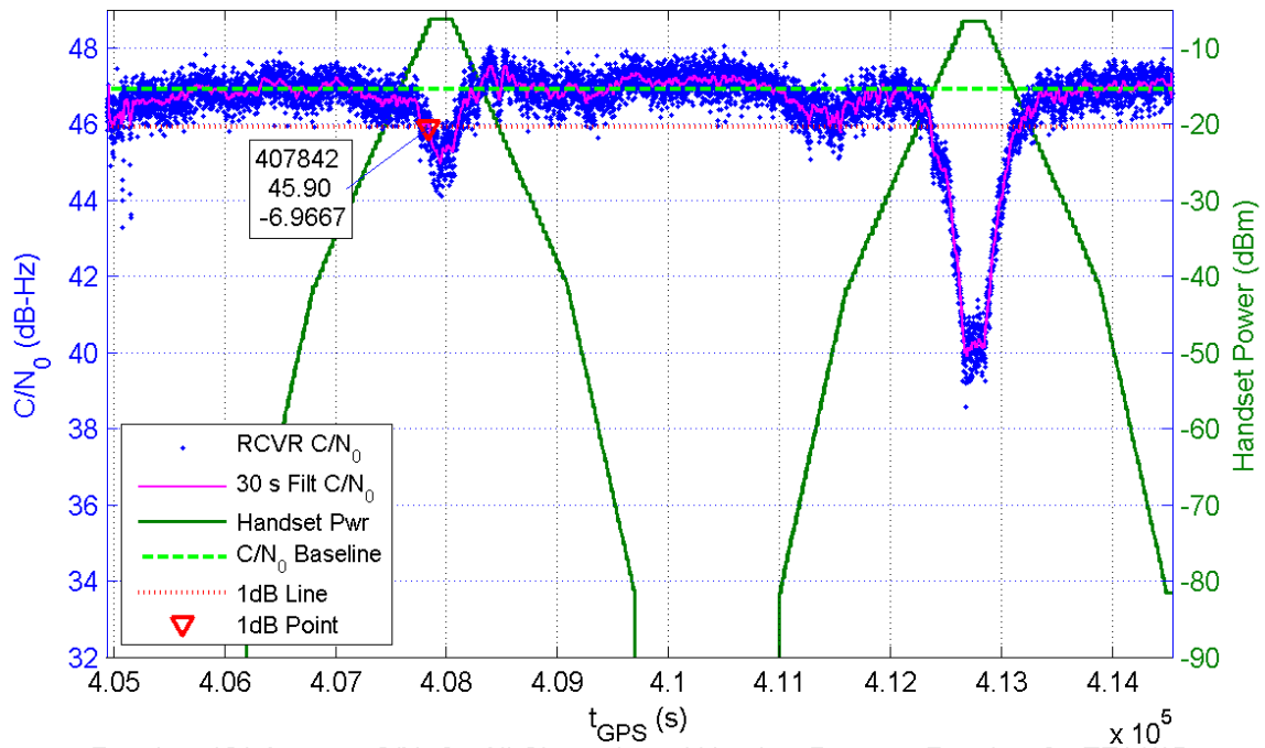
Receiver 121 Average C/N_0 for All Channels and Handset Power at Receiver for TE14/15
