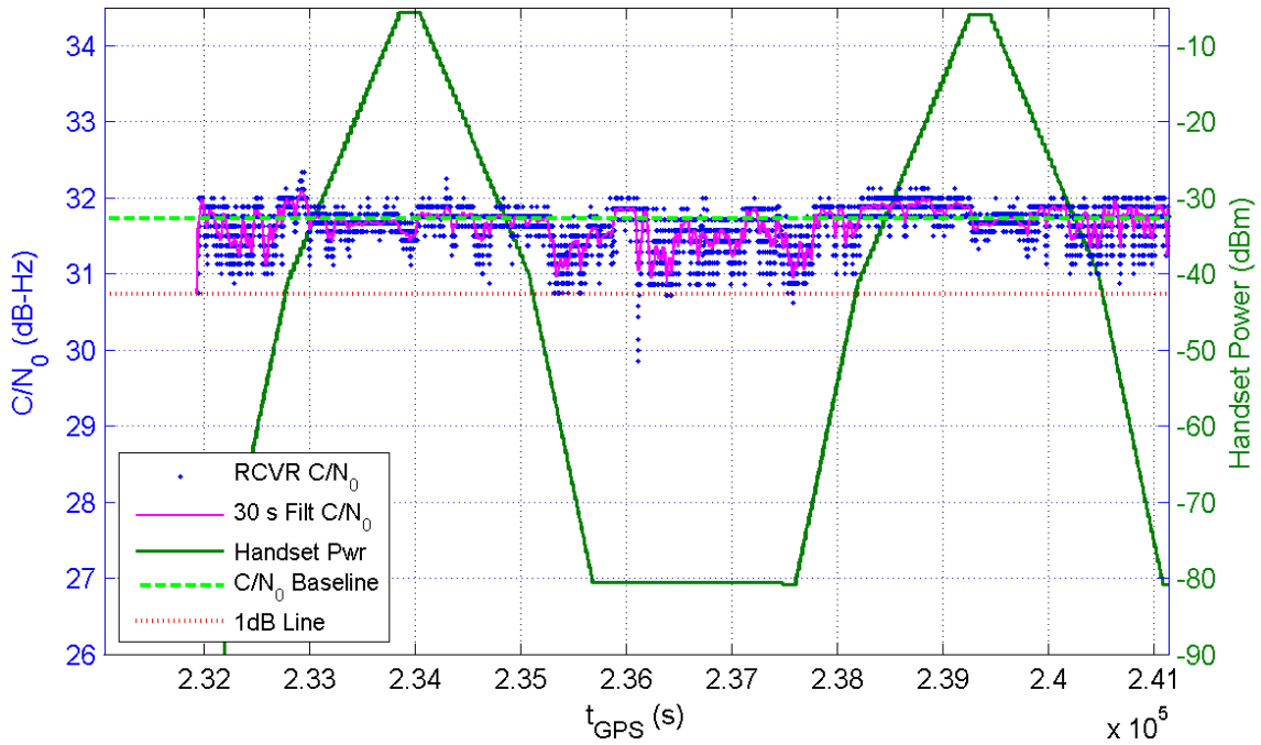
Receiver 322 Average C/N_0 for All Channels and Handset Power at Receiver for TE5/6
