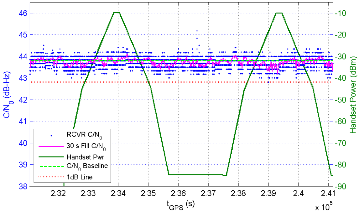
Receiver 393 Average C/N_0 for All Channels and Handset Power at Receiver for TE5/6
