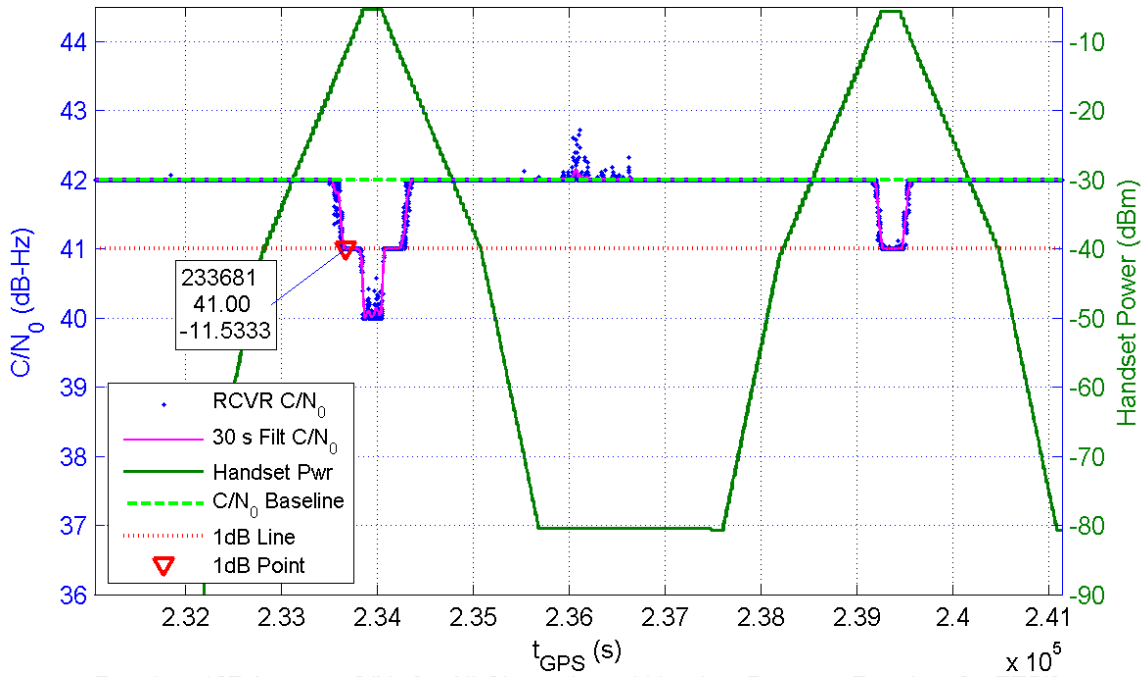
Receiver 107 Average C/N_0 for All Channels and Handset Power at Receiver for TE5/6
