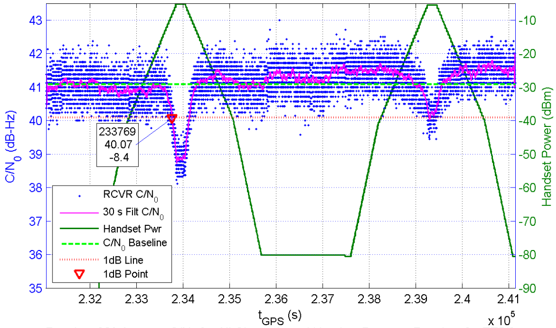
Receiver 328 Average C/N_0 for All Channels and Handset Power at Receiver for TE5/6
