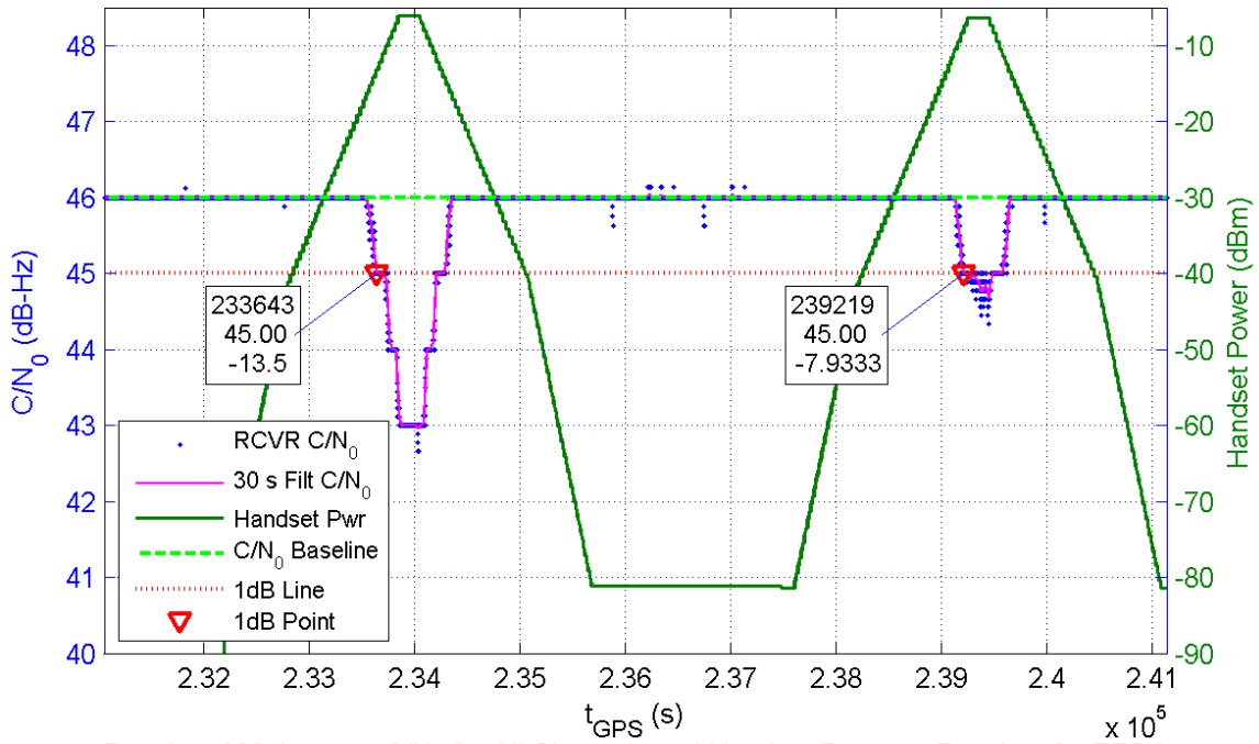
Receiver 333 Average C/N_0 for All Channels and Handset Power at Receiver for TE5/6
