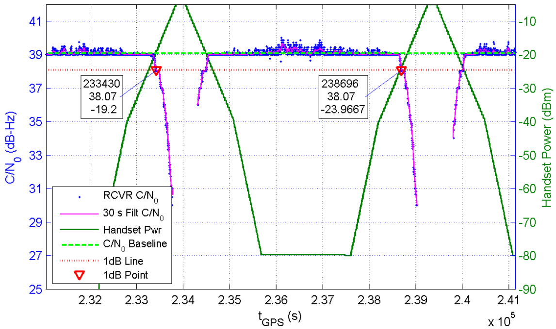
Receiver 328 Average C/N_0 for All Channels and Handset Power at Receiver for TE5/6
