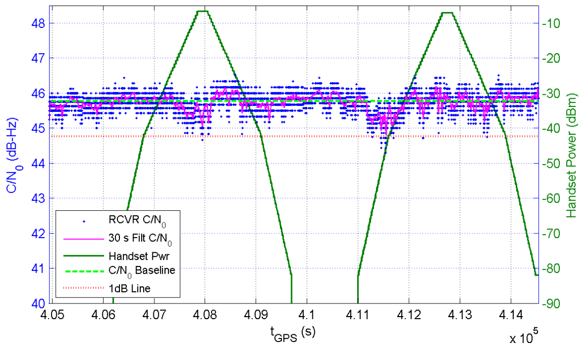
Receiver 396 Average C/N_0 for All Channels and Handset Power at Receiver for TE14/15
