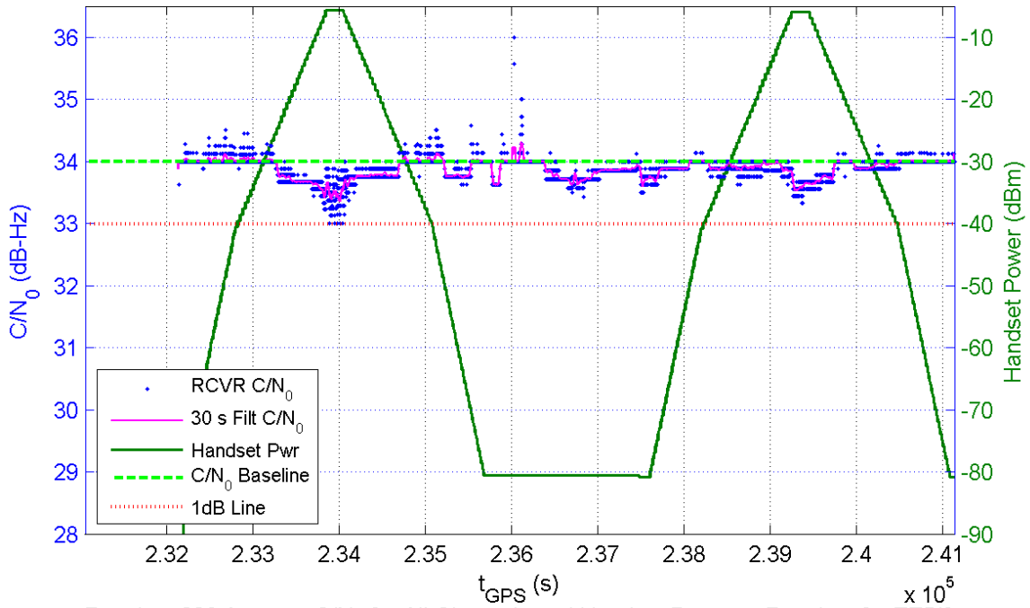
Receiver 206 Average C/N_0 for All Channels and Handset Power at Receiver for TE5/6
