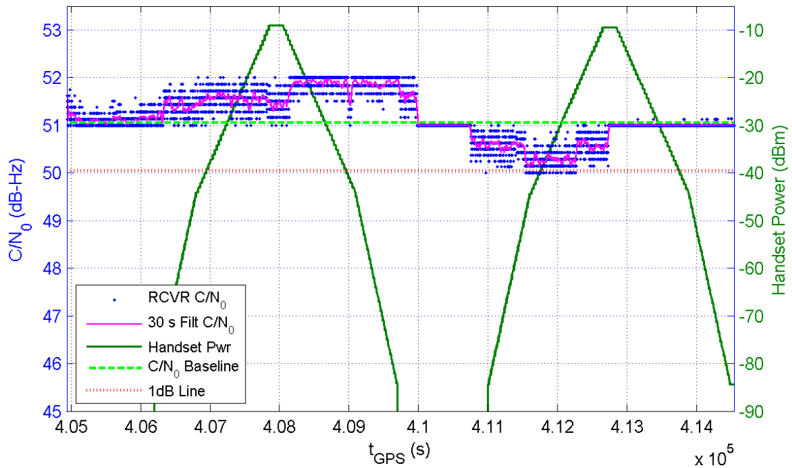
Receiver 108 Average C/N_0 for All Channels and Handset Power at Receiver for TE14/15
