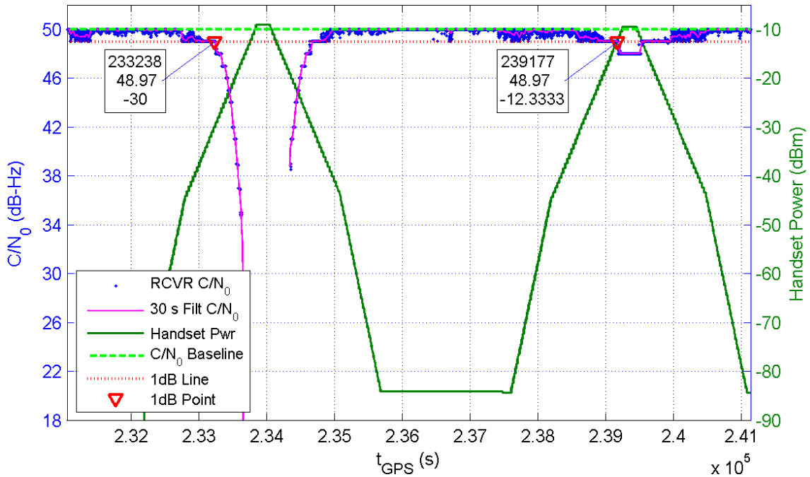
Receiver 351 Average C/N_0 for All Channels and Handset Power at Receiver for TE5/6
