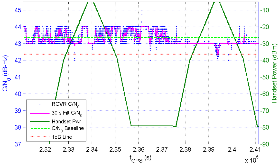
Receiver 369 Average C/N_0 for All Channels and Handset Power at Receiver for TE5/6
