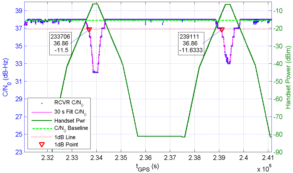
Receiver 320 Average C/N_0 for All Channels and Handset Power at Receiver for TE5/6
