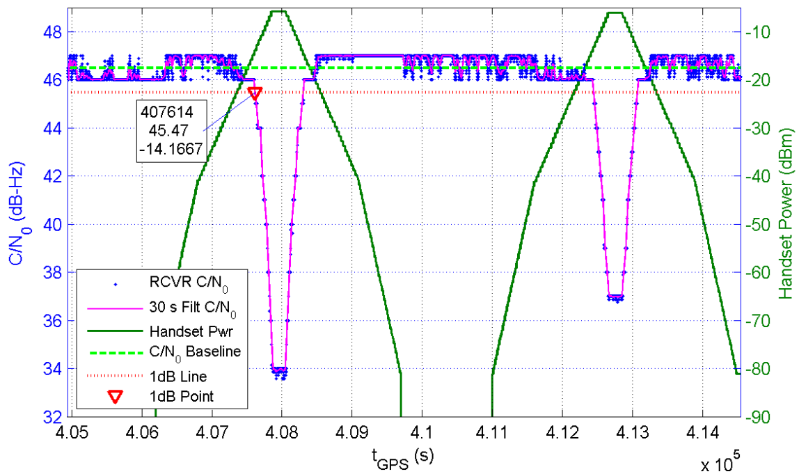
Receiver 205 Average C/N_0 for All Channels and Handset Power at Receiver for TE14/15
