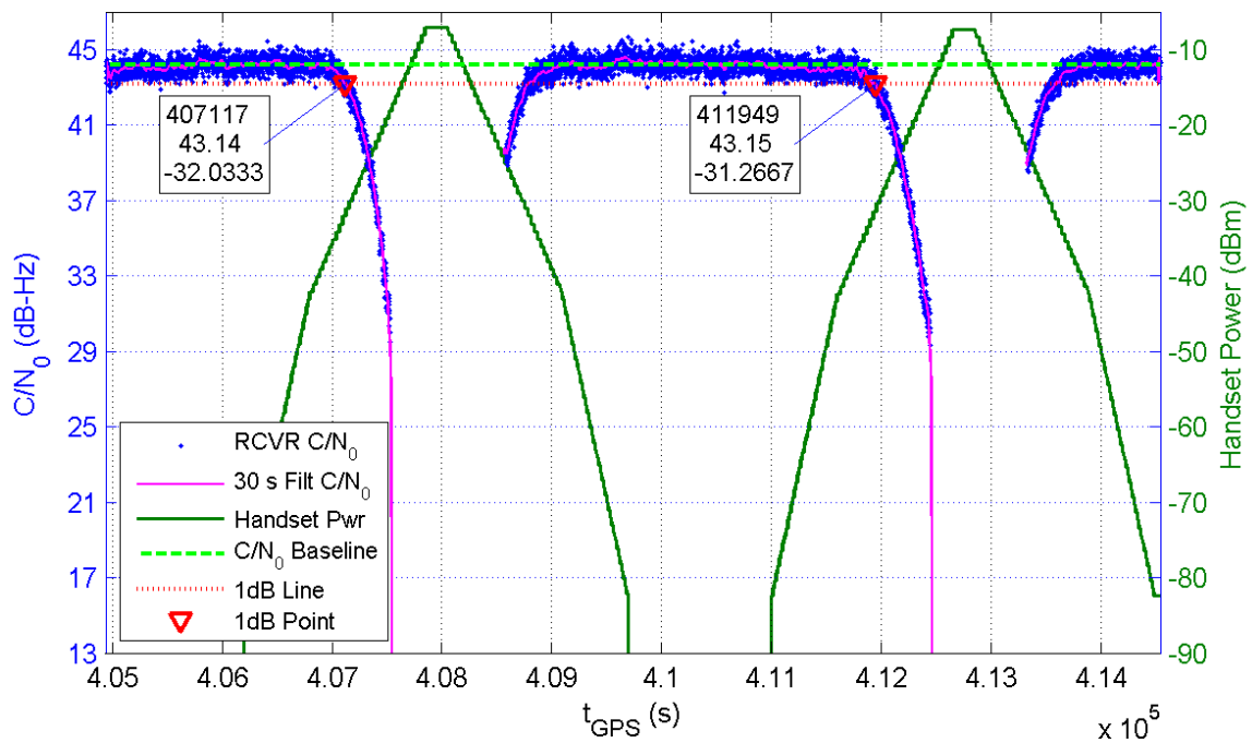
Receiver 235 Average C/N_0 for All Channels and Handset Power at Receiver for TE14/15
