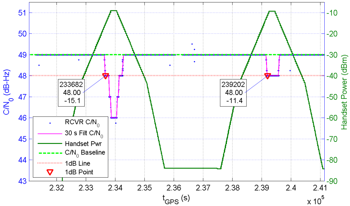
Receiver 379 Average C/N_0 for All Channels and Handset Power at Receiver for TE5/6
