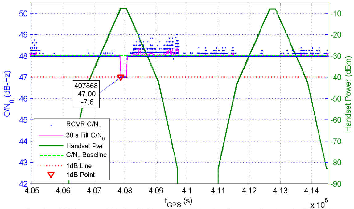
Receiver 306 Average C/N_0 for All Channels and Handset Power at Receiver for TE14/15
