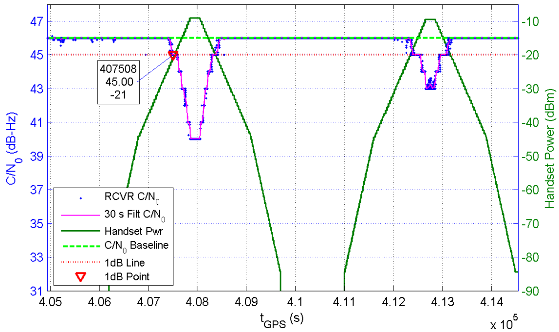
Receiver 333 Average C/N_0 for All Channels and Handset Power at Receiver for TE14/15
