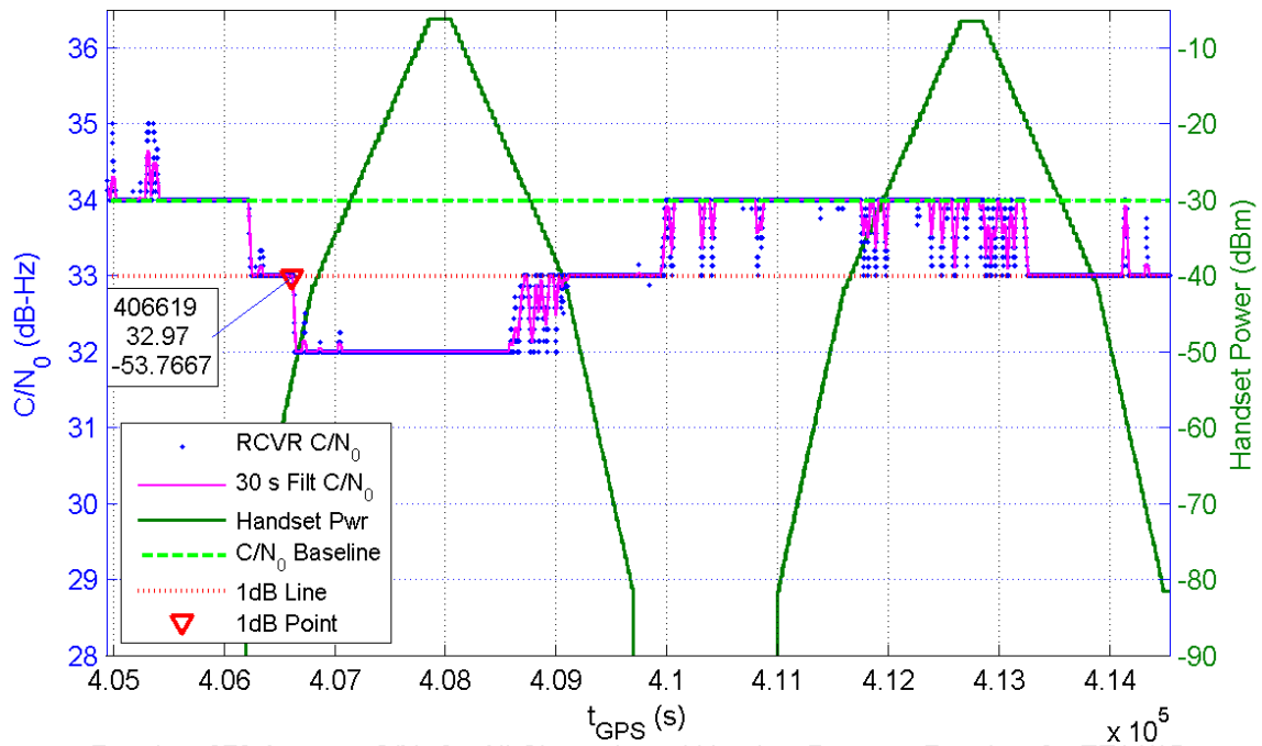
Receiver 379 Average C/N_0 for All Channels and Handset Power at Receiver for TE14/15
