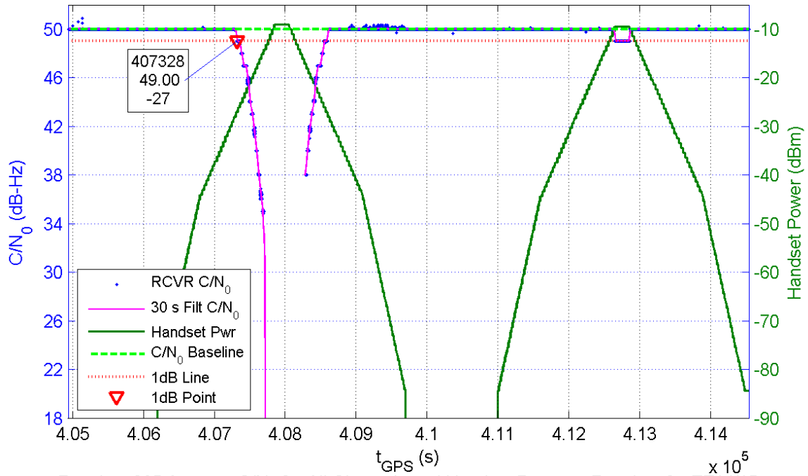
Receiver 385 Average C/N_0 for All Channels and Handset Power at Receiver for TE14/15
