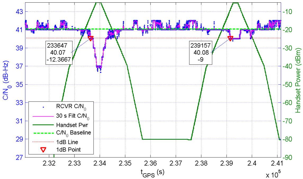
Receiver 134 Average C/N_0 for All Channels and Handset Power at Receiver for TE5/6
