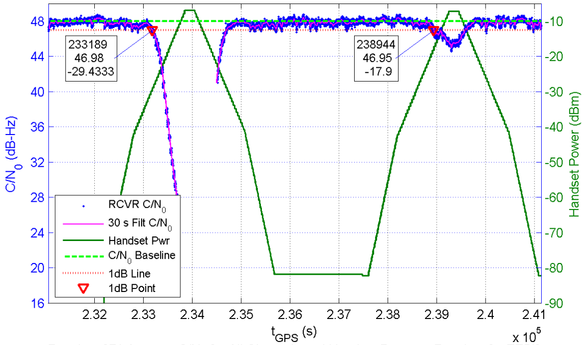
Receiver 371 Average C/N_0 for All Channels and Handset Power at Receiver for TE5/6
