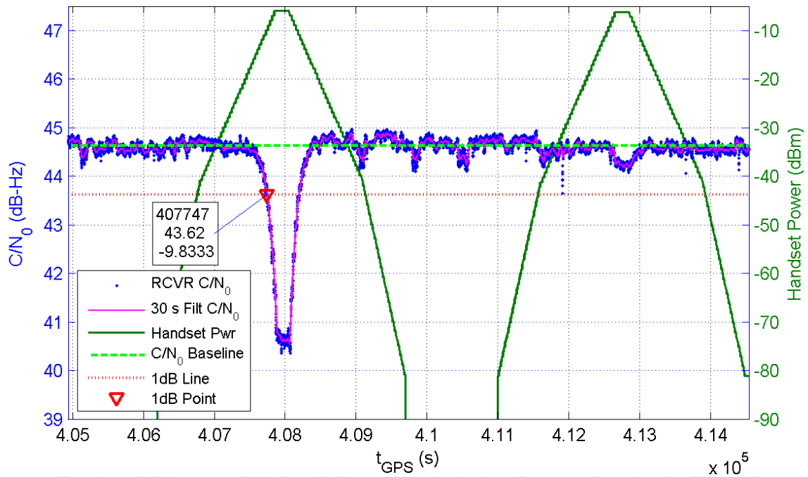
Receiver 317 Average C/N 0 for All Channels and Handset Power at Receiver for TE14/15
