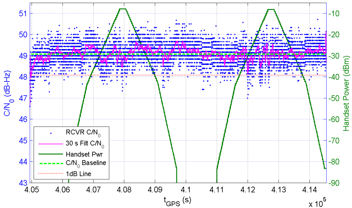
Receiver 363 Average C/N 0 for All Channels and Handset Power at Receiver for TE14/15
