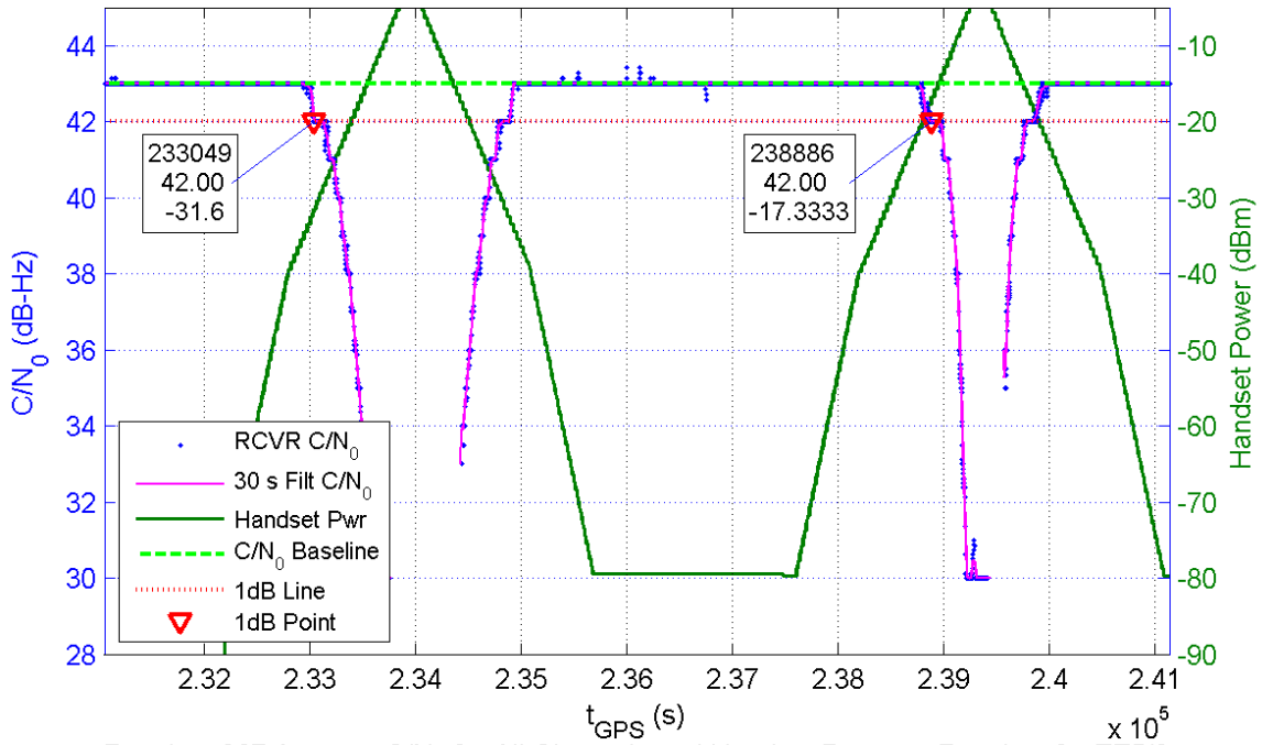
Receiver 367 Average C/N_0 for All Channels and Handset Power at Receiver for TE5/6
