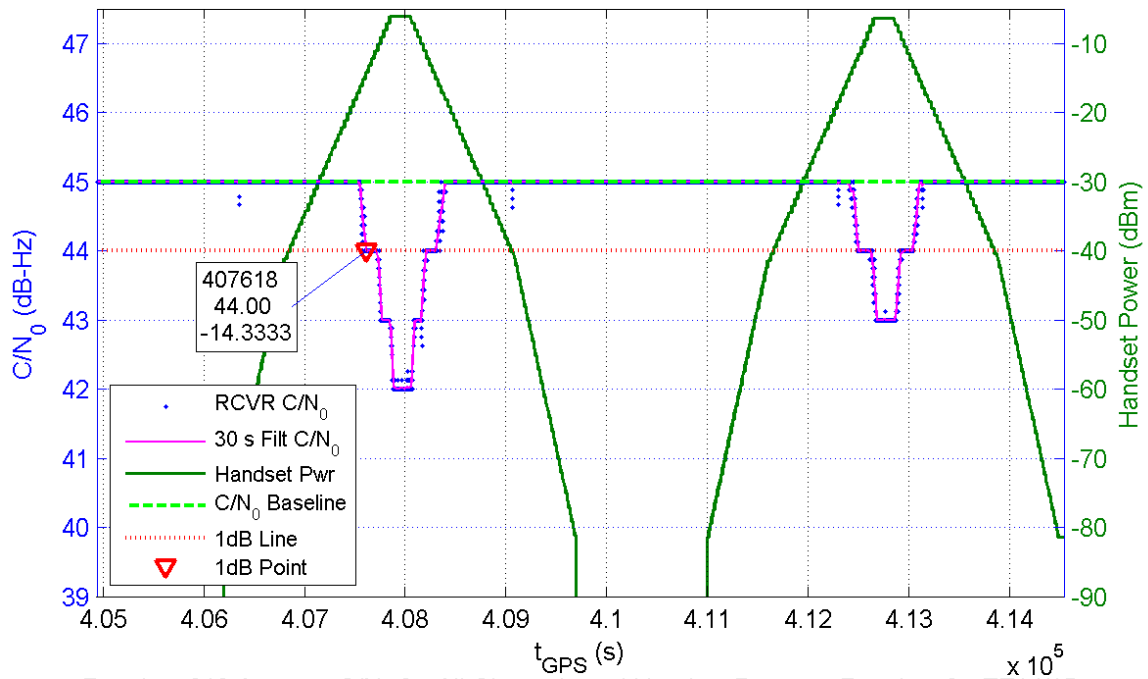
Receiver 319 Average C/N_0 for All Channels and Handset Power at Receiver for TE14/15
