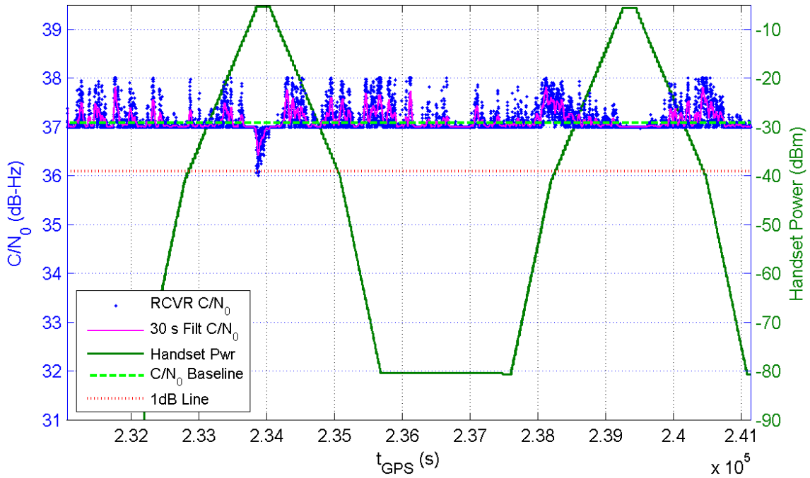
Receiver 383 Average C/N_0 for All Channels and Handset Power at Receiver for TE5/6
