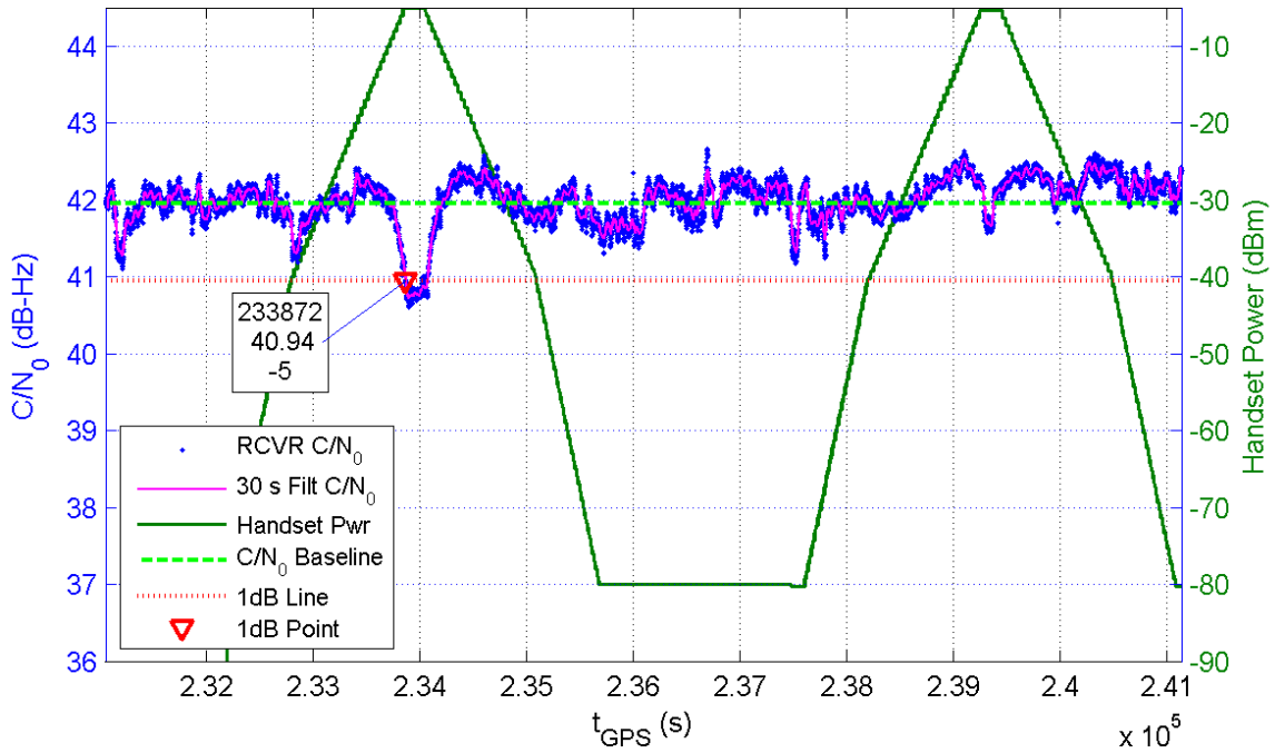
Receiver 342 Average C/N_0 for All Channels and Handset Power at Receiver for TE5/6
