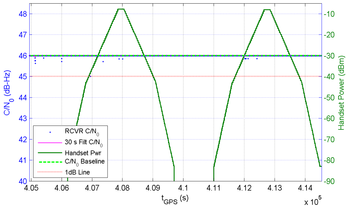
Receiver 319 Average C/N_0 for All Channels and Handset Power at Receiver for TE14/15
