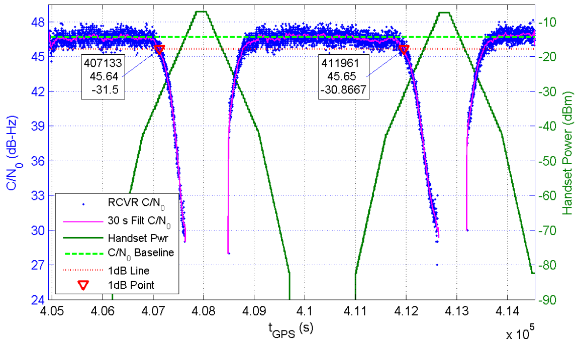
Receiver 247 Average C/N_0 for All Channels and Handset Power at Receiver for TE14/15
