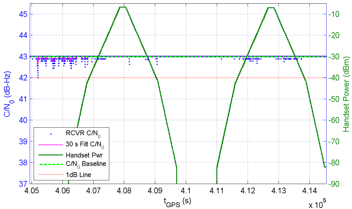
Receiver 354 Average C/N_0 for All Channels and Handset Power at Receiver for TE14/15
