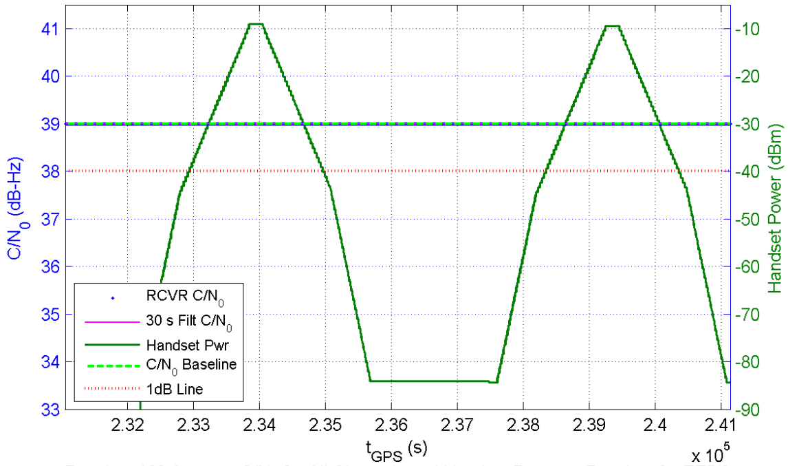
Receiver 129 Average C/N_0 for All Channels and Handset Power at Receiver for TE5/6
