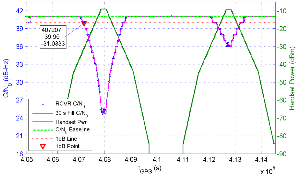
Receiver 351 Average C/N_0 for All Channels and Handset Power at Receiver for TE14/15
