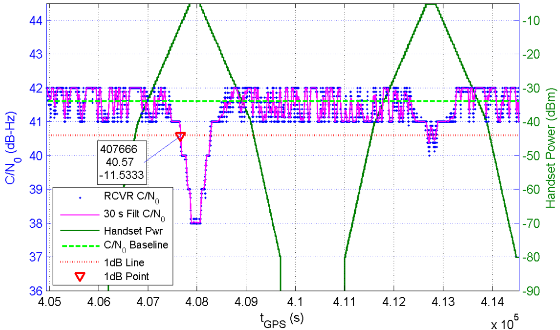
Receiver 104 Average C/N_0 for All Channels and Handset Power at Receiver for TE14/15
