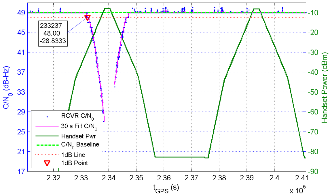
Receiver 109 Average C/N_0 for All Channels and Handset Power at Receiver for TE5/6
