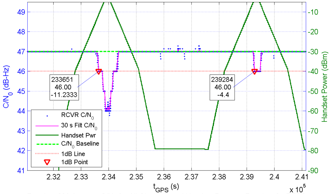
Receiver 338 Average C/N_0 for All Channels and Handset Power at Receiver for TE5/6
