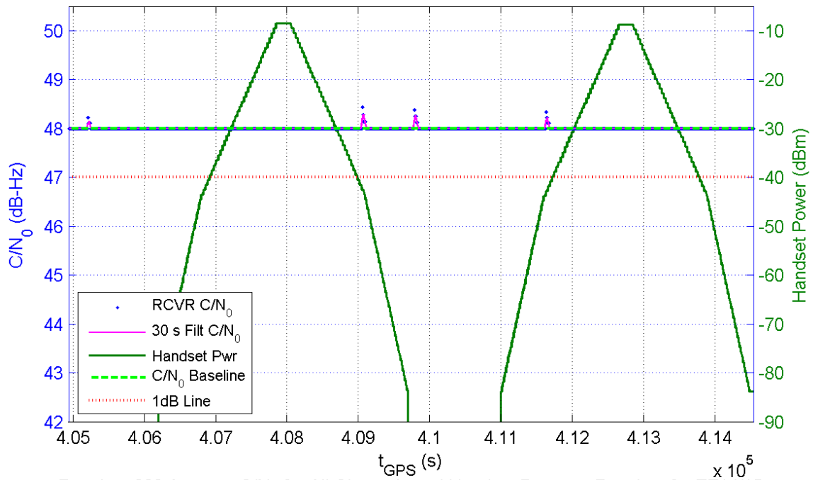
Receiver 220 Average C/N_0 for All Channels and Handset Power at Receiver for TE14/15
