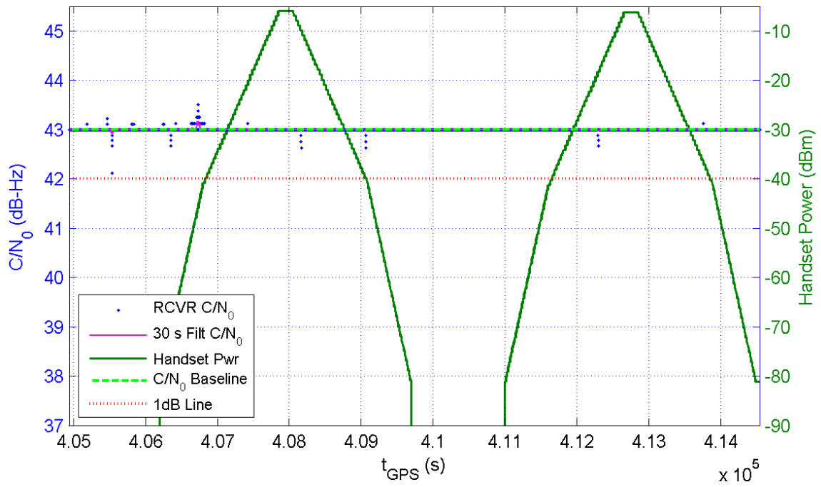
Receiver 397 Average C/N_0 for All Channels and Handset Power at Receiver for TE14/15
