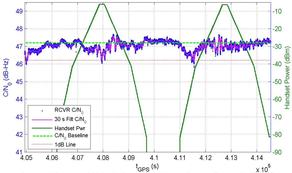
Receiver 235 Average C/N_0 for All Channels and Handset Power at Receiver for TE14/15
