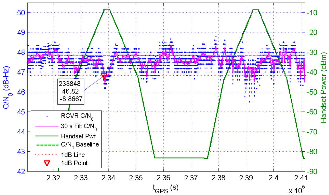
Receiver 123 Average C/N_0 for All Channels and Handset Power at Receiver for TE5/6
