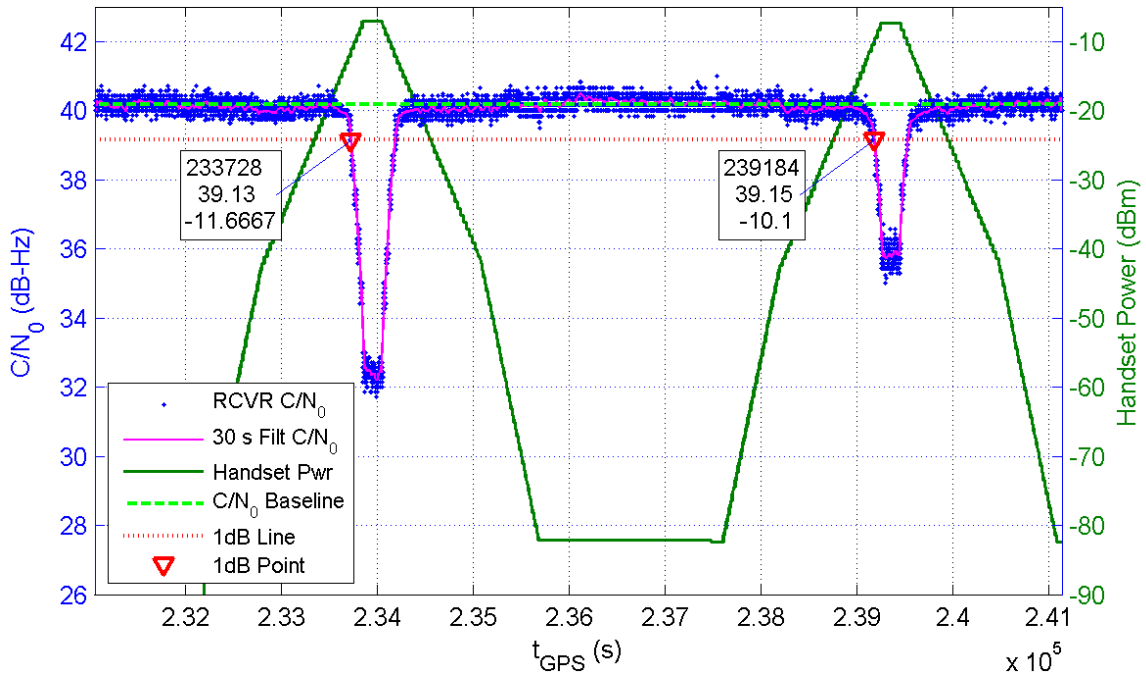
Receiver 374 Average C/N_0 for All Channels and Handset Power at Receiver for TE5/6
